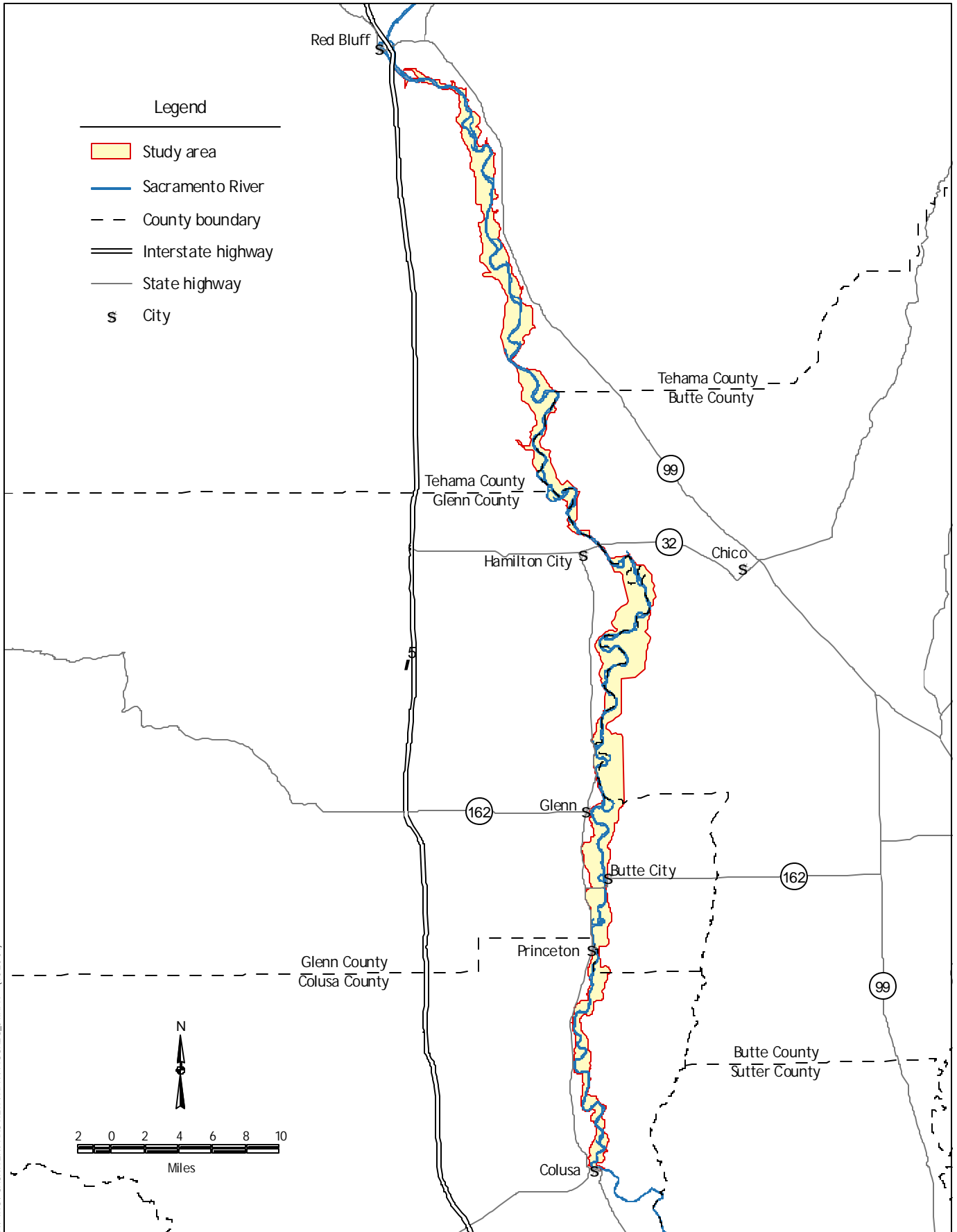
Figure 4-2 Study Area Vicinity Map
