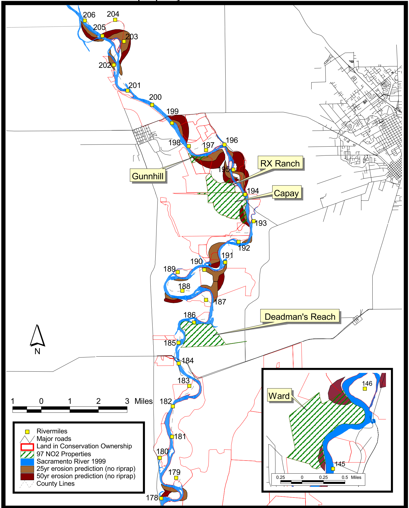
Appendix 6. Figure 4. Predicted erosion among the Chico Landing Subreach and the Ward property.
