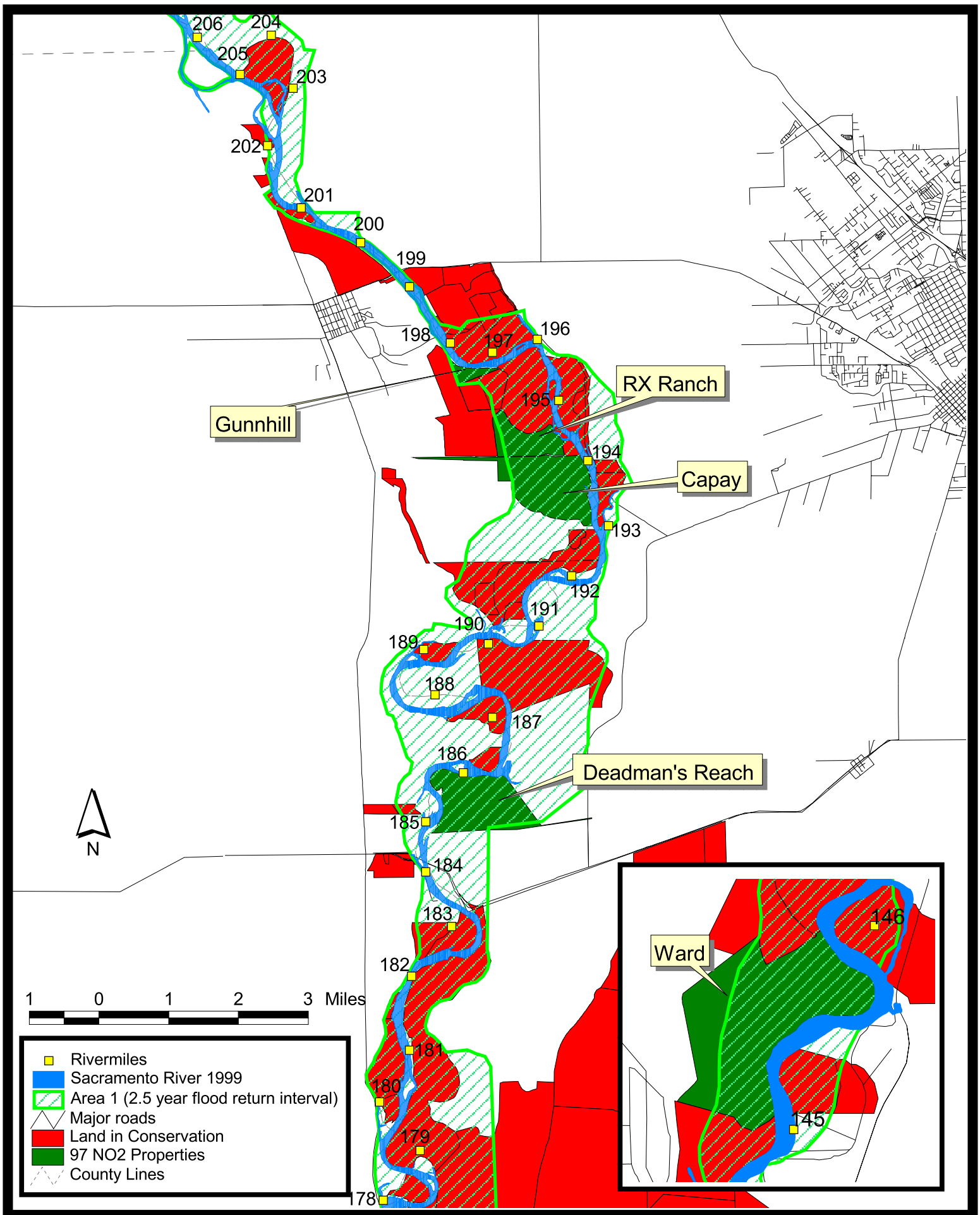
Appendix 6. Figure 2. Frequent flooding among the Chico Landing Subreach and Ward Property (2.5 year return interval flood).
