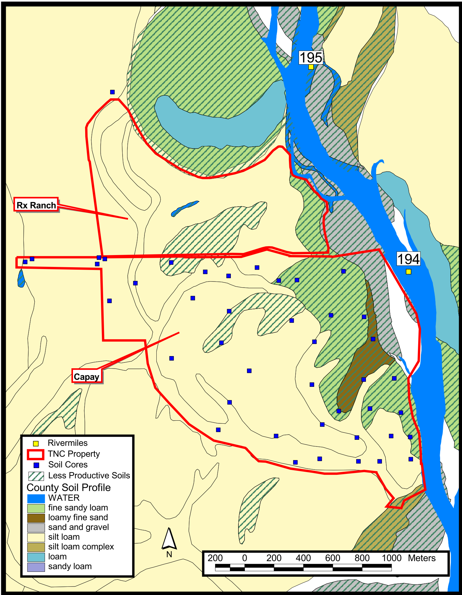
Appendix 2. Figure 2B. RX Ranch and Capay soil profiles.
