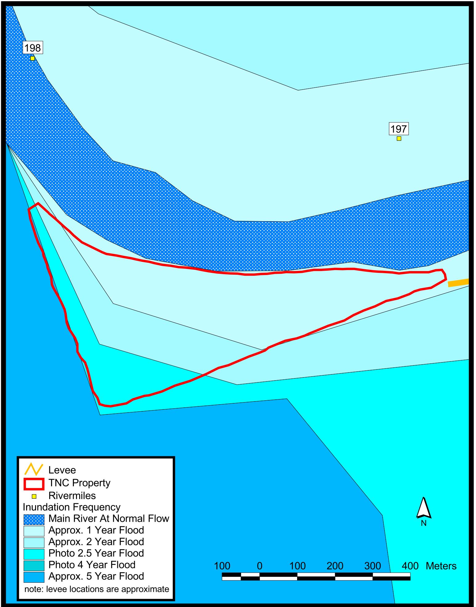
Appendix 2. Figure 1C. Gunnhill flood frequencies.
