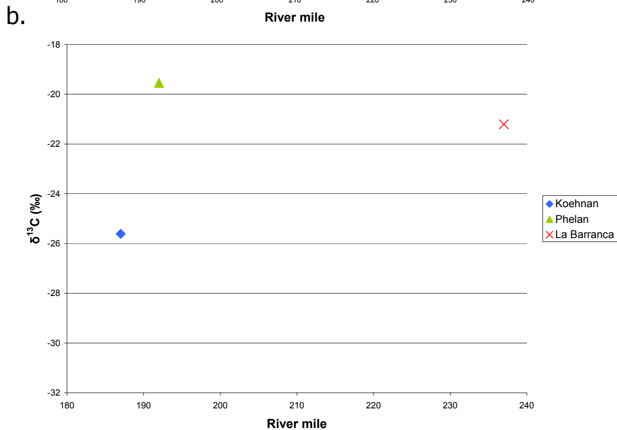
Figure 5-7. Stable isotope signatures for aquatic vegetation and algae for (a) nitrogen and (b) carbon.
