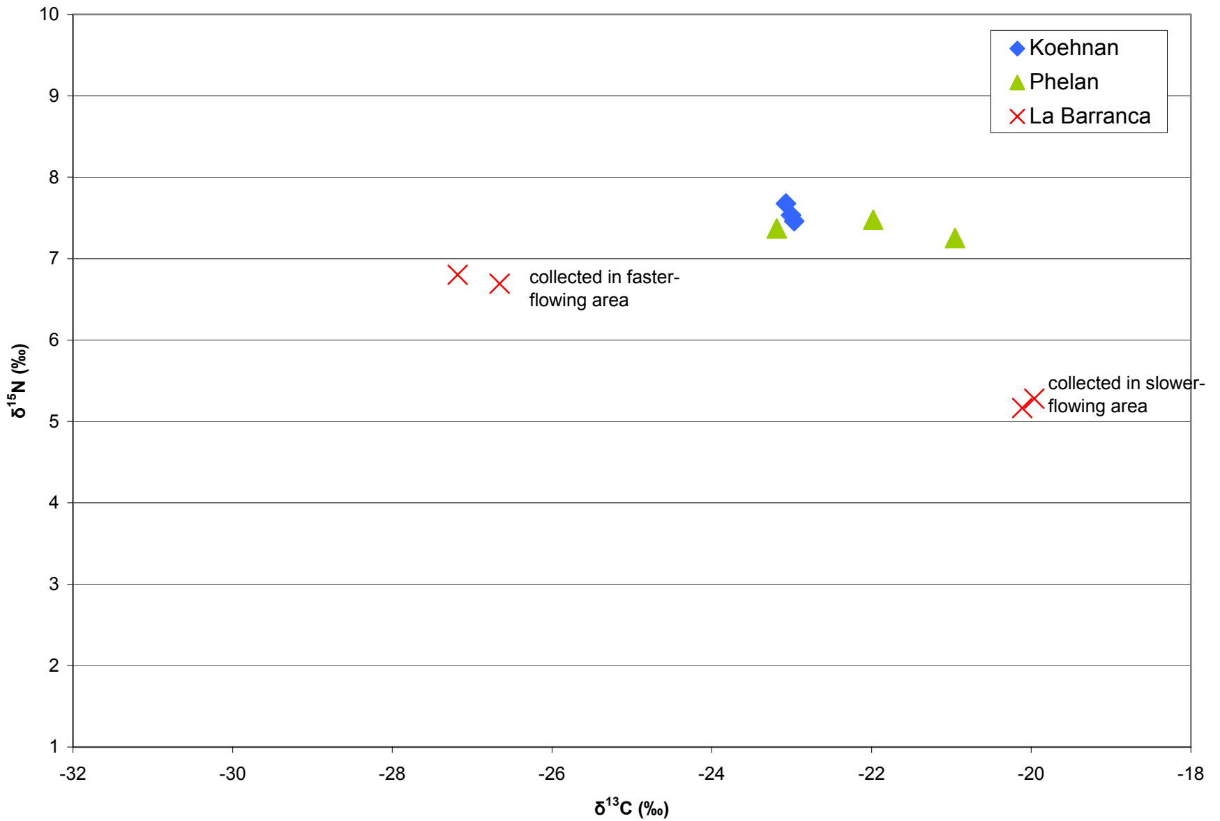
Figure 5-4. Dual isotope diagram for grazers (mayflies).
