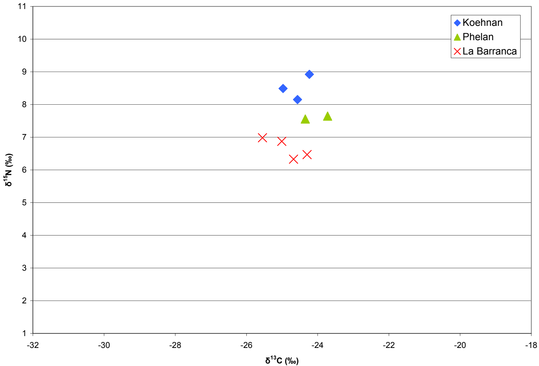
Figure 5-2. Dual isotope diagram for filter-feeders (Hydropsychids and blackflies).
