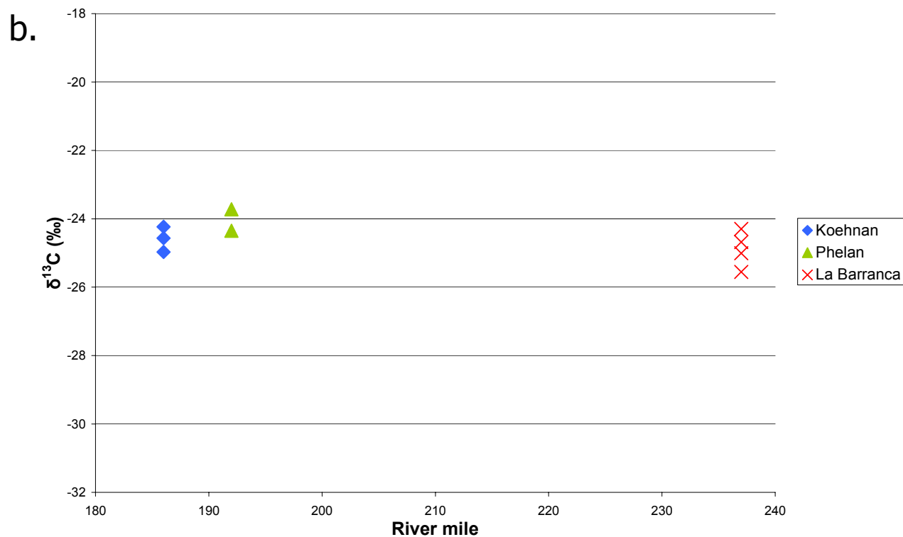
Figure 5-1. Stable isotope signatures for filter-feeders (hydropsychids and blackflies) for (a) nitrogen and (b) carbon.
