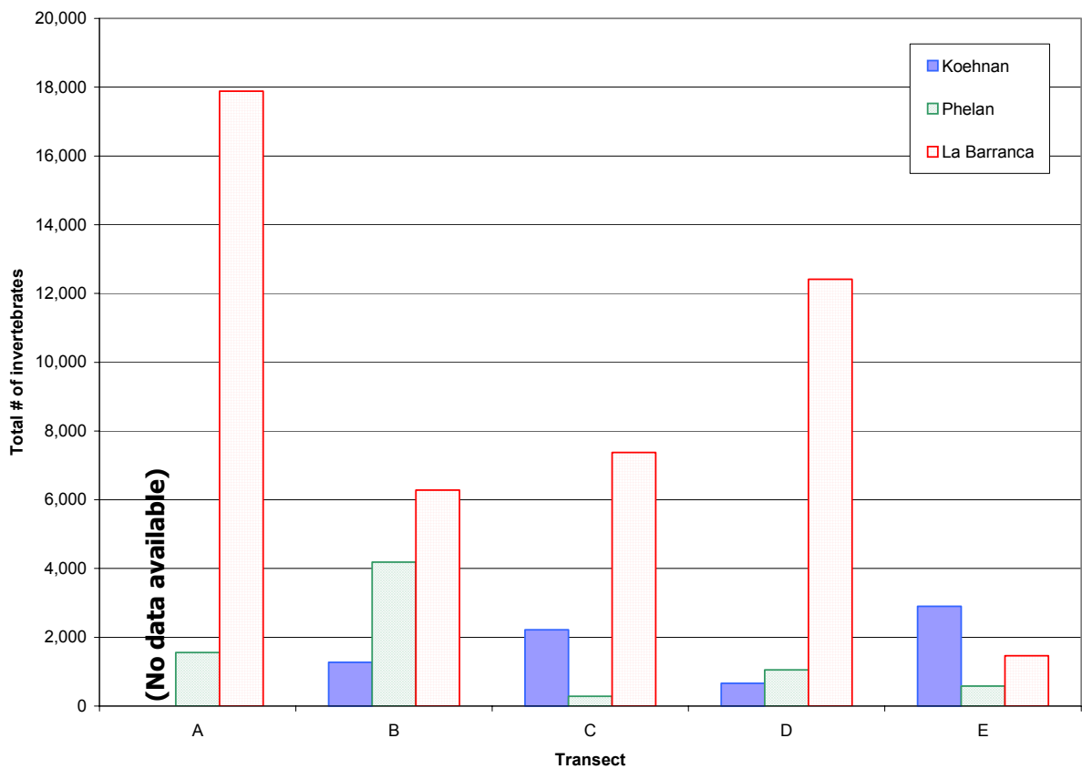
Figure 4-7. Invertebrate abundance (all taxa) captured at study sites (A is the upstream-most transect, E is downstream-most transect).
