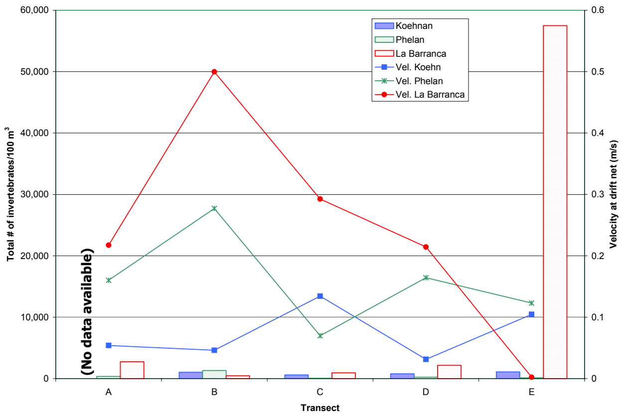
Figure 4-8. Invertebrate abundance (all taxa) captured at study sites (corrected for volume of flow sampled) and velocity at sampling locations (A is the upstream-most transect, E is downstream-most transect).
