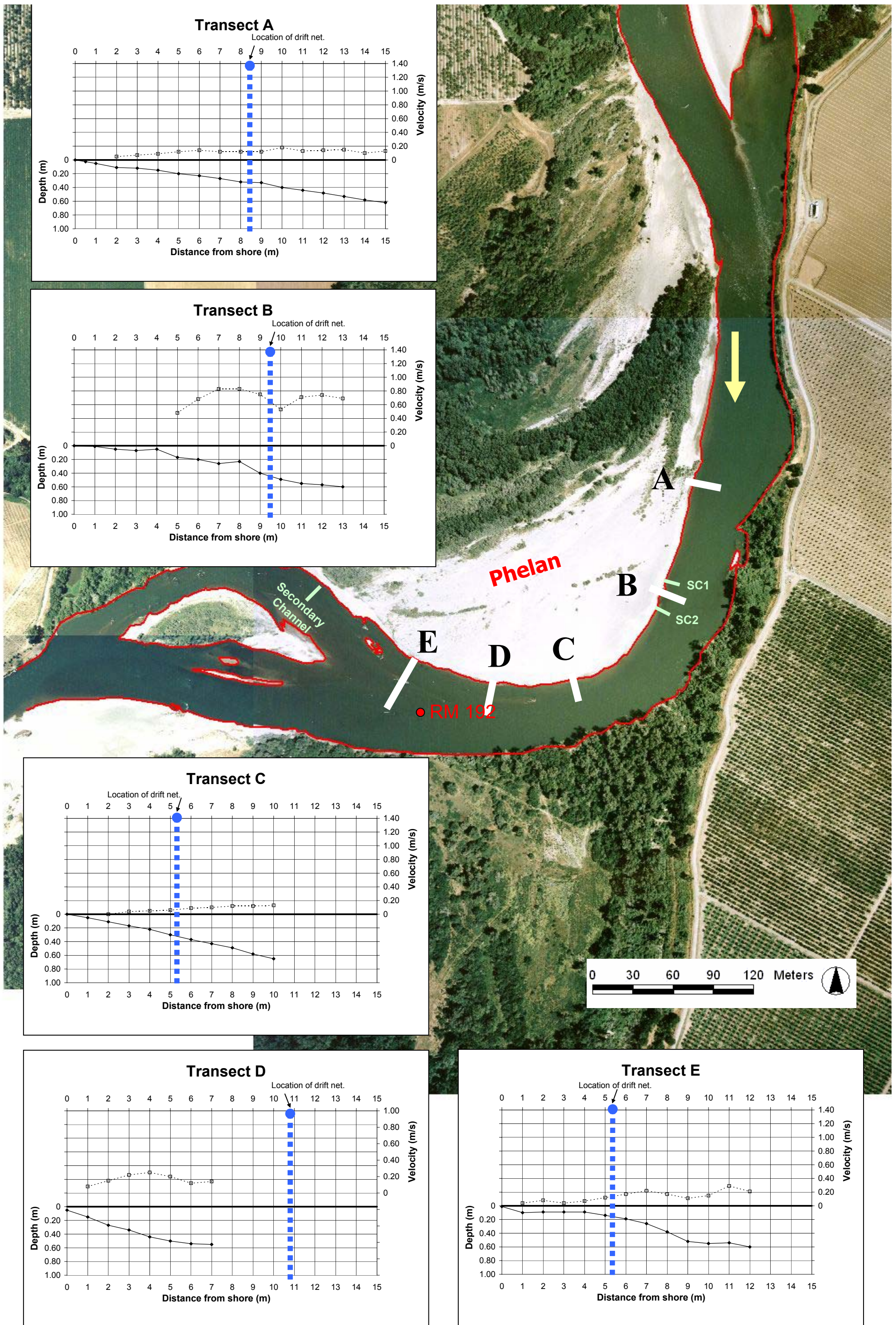
Figure 4-5. Phelan site map with velocity and depth profiles for the five transects along the point bar. Each dot along the graph designates a sampling point. Depth and velocity measurements were typically taken every 0.5 m with some exception at longer transects. SC1 and SC2 designate cove habitat sampling locations, and Secondary Channel refers to secondary channel sampling site.
