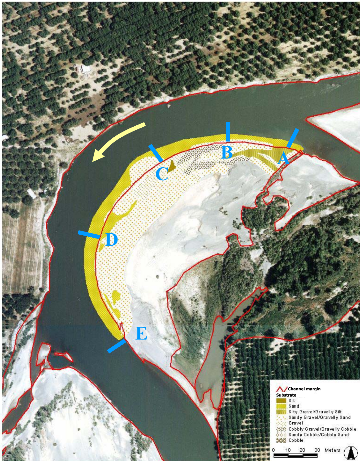
Figure 4-3. (a) Substrate composition and (b) facies mapping data along the five transects at the Koehnan point bar. The red outline is an outline of the wetted channel. Direction of flow is indicated by the arrow. This point bar occurs between RM 185 and 186.
