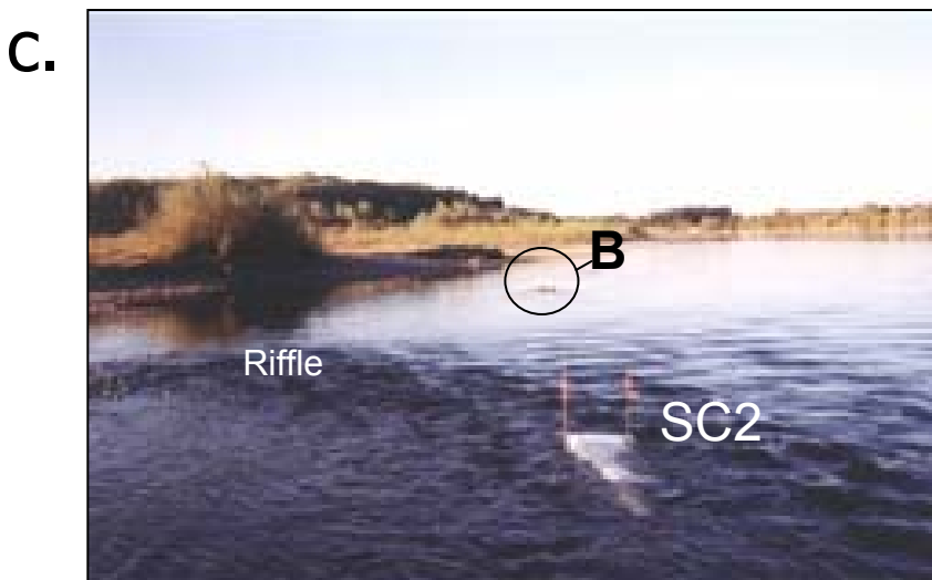
Figure 4-21. Cove habitat sampling locations at the Phelan point bar. a) Diagram of cove habitat and net locations. b) View of SC1 looking upstream. c) View of SC2 looking upstream with Transect B in the background.
