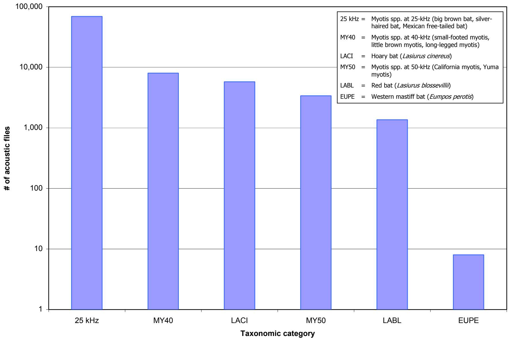
Figure 3-9. Total number of acoustic files by taxonomic category at the Koehnan backwater sampling location.
