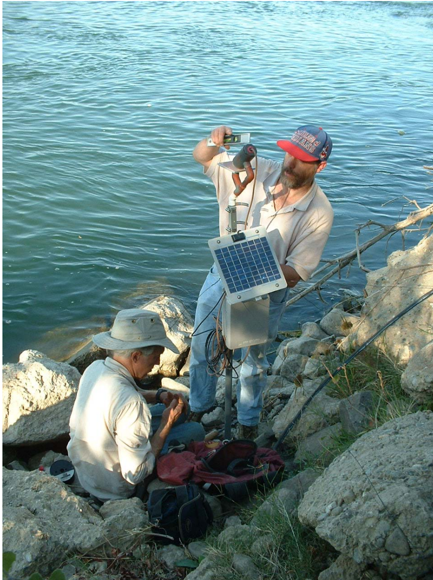
Figure 3-5. Detector deployment and setup example. (a) The Koehnan mainstem Sacramento River site. (b) Close up of detector components.
