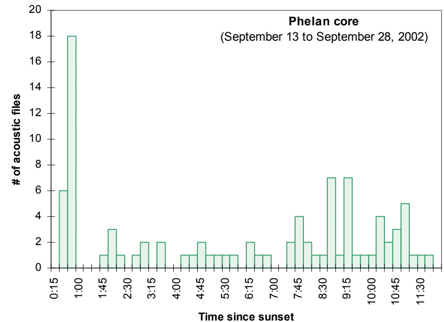
Figure 3-32. Distribution of acoustic files since sunset for red bats at the 2002 and 1991 restoration sites, and the Phelan core sampling location. September 13 to October 21, 2002 refers to the entire study period, and September 13 to September 28, 2002 refers to the restoration plot study period only. For any instance of estimated time since emergence of less than 1 hour, that time, and an estimate of straight-line travel distance (using flight speed of 5 meters per second) is shown for an approximate scale of distances to roost sites.
