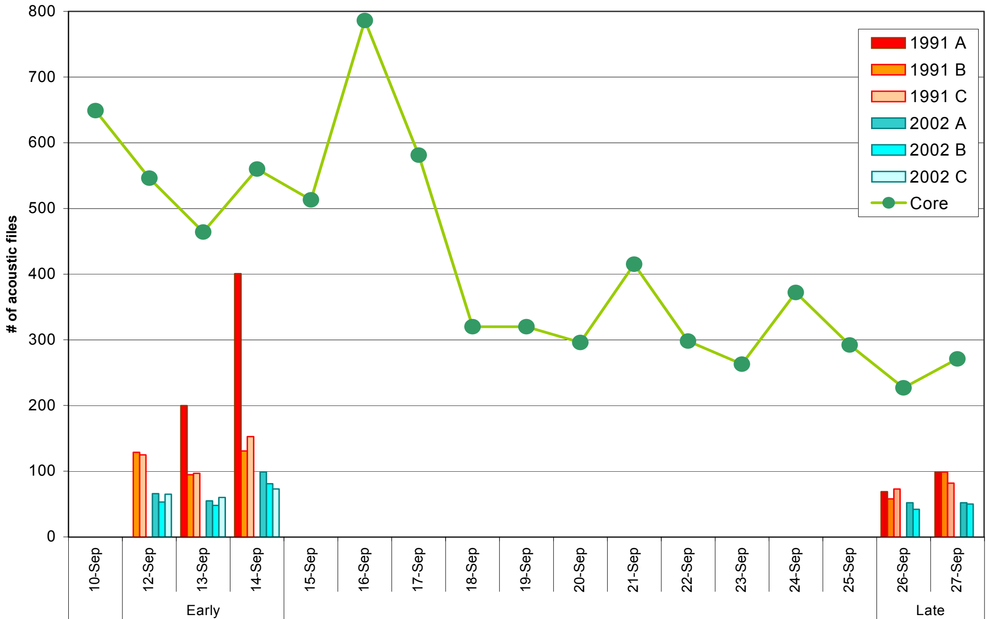
Figure 3-29. Number of acoustic files at 2002 and 1991 restoration sites (bars), and at the Phelan core sampling location (line). “Early” refers to the September 12–14, 2002 sampling period (solid colored bars), and “Late” refers to the September 26–27, 2002 sampling period (bars with colored grids). At each site, detectors were deployed at three locations (A, B, C).
