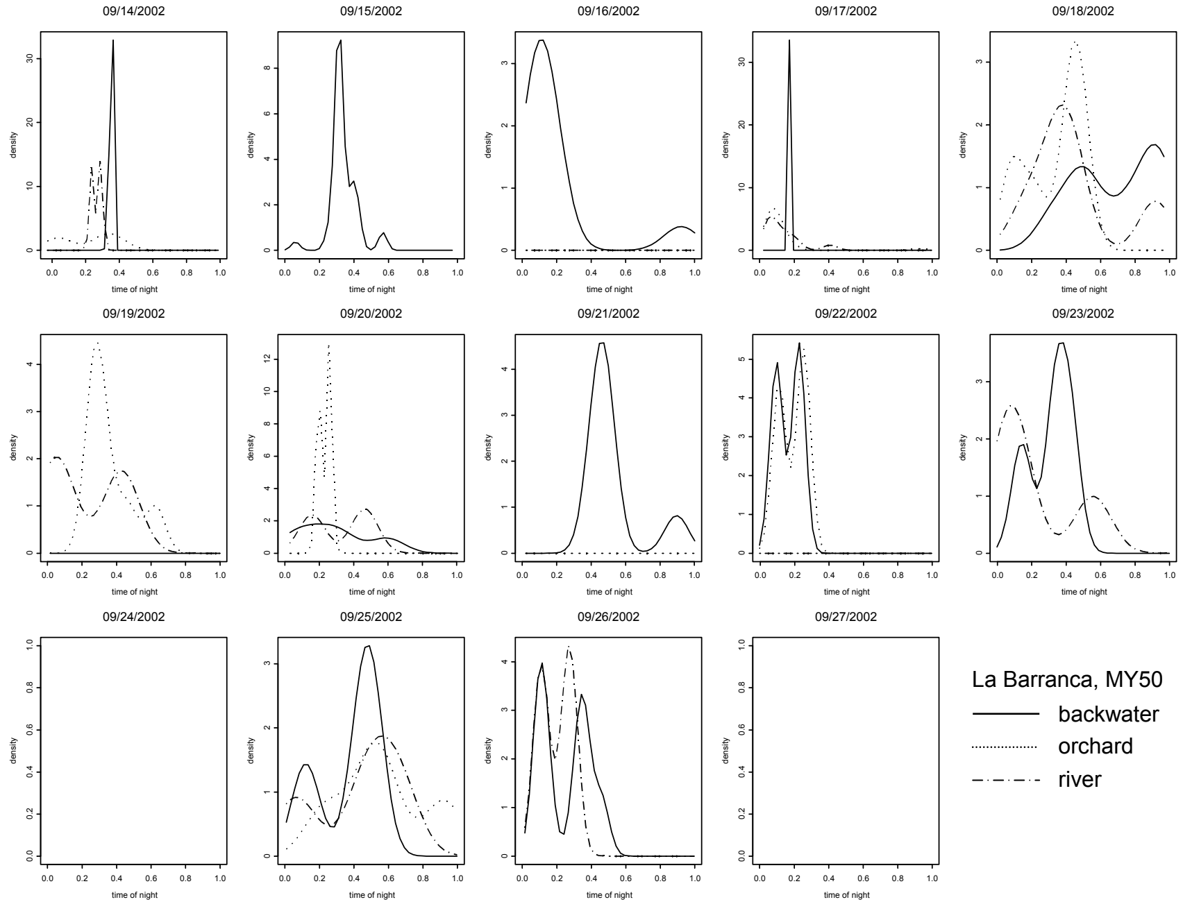
Figure 3-24. 40-kHz Myotis phenotype at La Barranca sampling location during the first two weeks of sampling (September 14-27). For the x-axis, 0 denotes sunset and 1.0 denotes sunrise, and has been corrected for the changing duration. The y-axis is a probability density for the time of acoustic detection, analogous to a smoothed and normalized histogram of acoustic detections.
