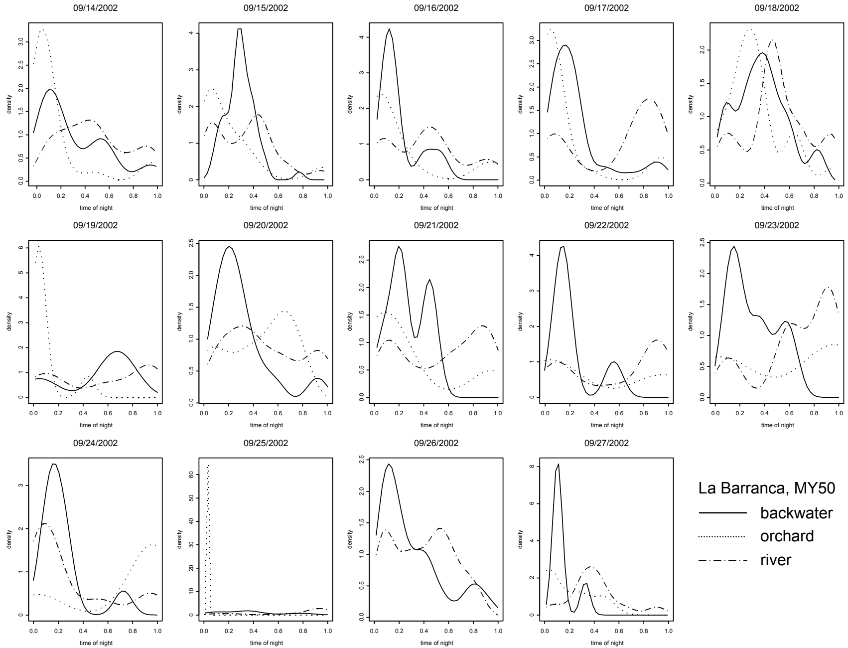
Figure 3-23. Records of 50-kHz Myotis phonotype at La Barranca sampling locations during the first two weeks of sampling (September 14-27). For the x-axis, 0 denotes sunset and 1.0 denotes sunrise, and has been corrected for the changing duration. The y-axis is a probability density for the time of acoustic detection, analogous to a smoothed and normalized histogram of acoustic detections.
