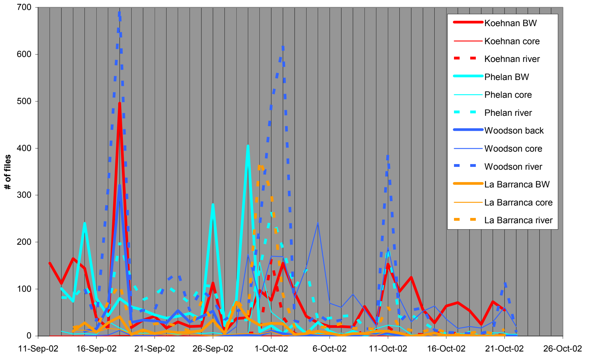
Figure 3-22. Total number of acoustic files per night of 50-kHz Myotis phenotype at study sites and sampling locations.
