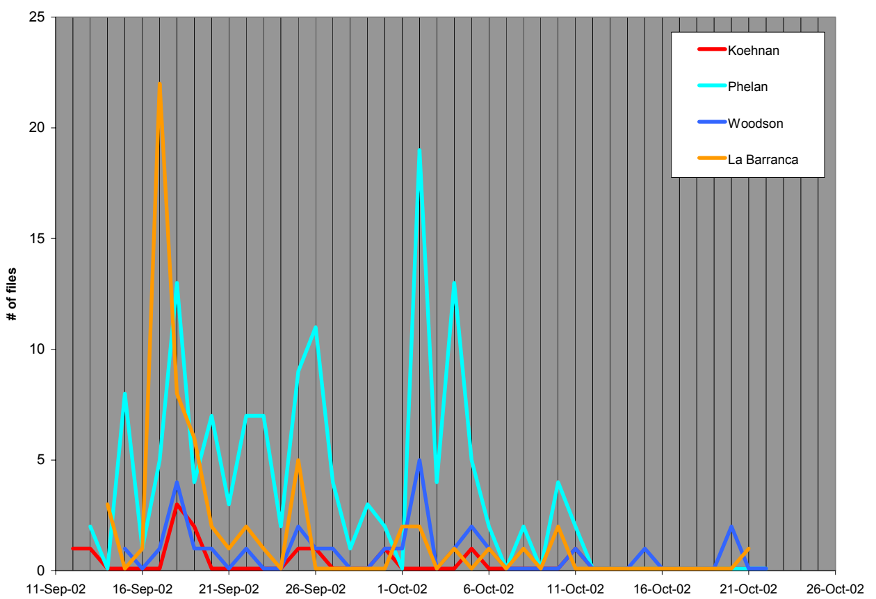
Figure 3-17. File counts per night of 40-kHz Myotis phenotype at core sampling locations.
