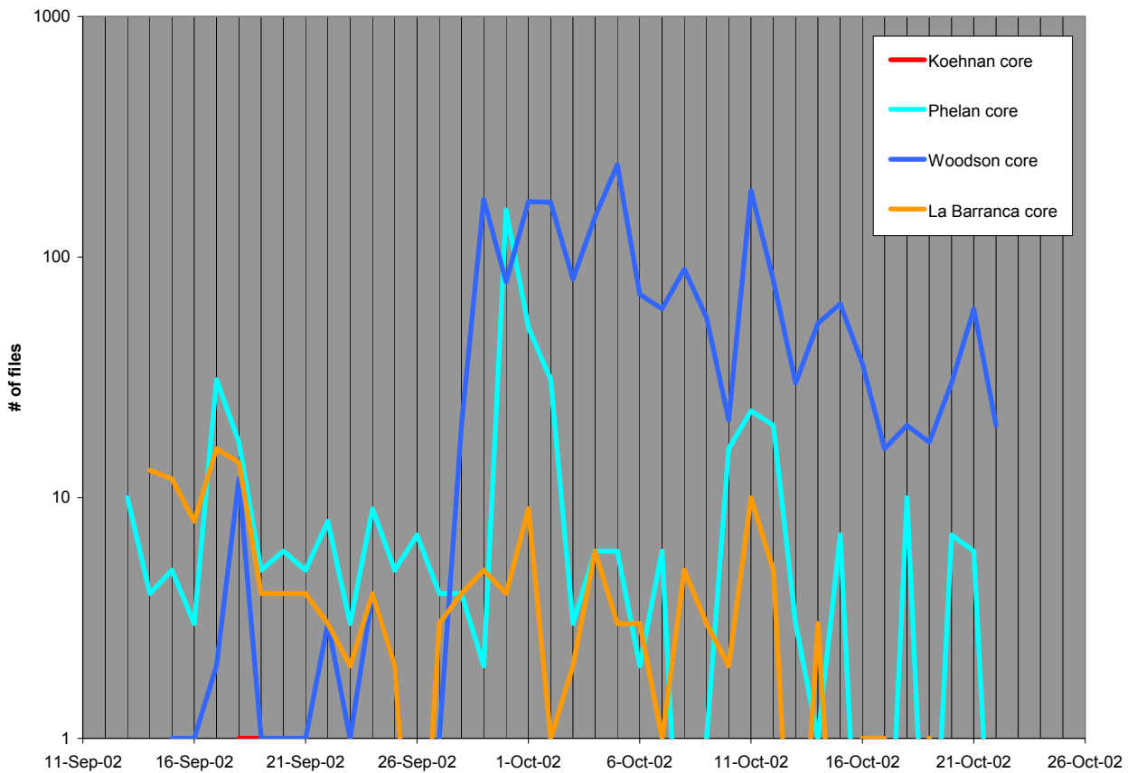
Figure 3-18. File counts per night of 50-kHz Myotis phenotype at core sampling locations. Note log scale on the y-axis.
