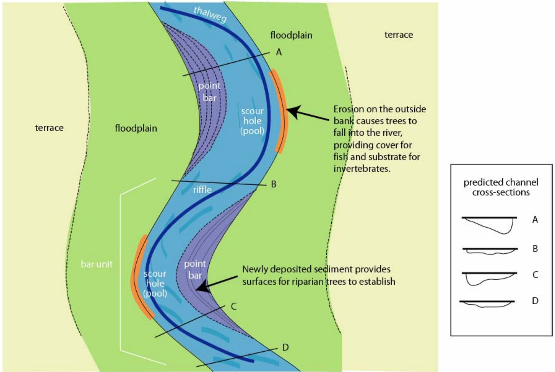
Figure 2-3. Predicted form and function of large meandering alluvial rivers.
