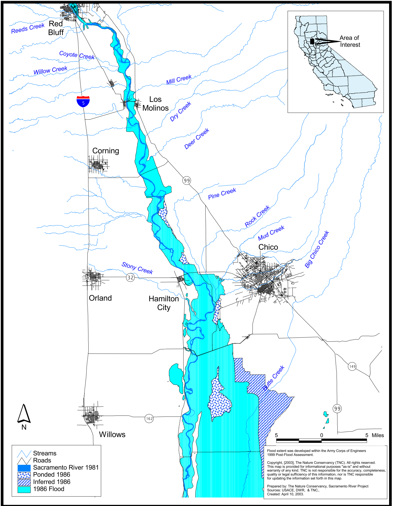
Figure 2b. Extent of flooding in 1986
