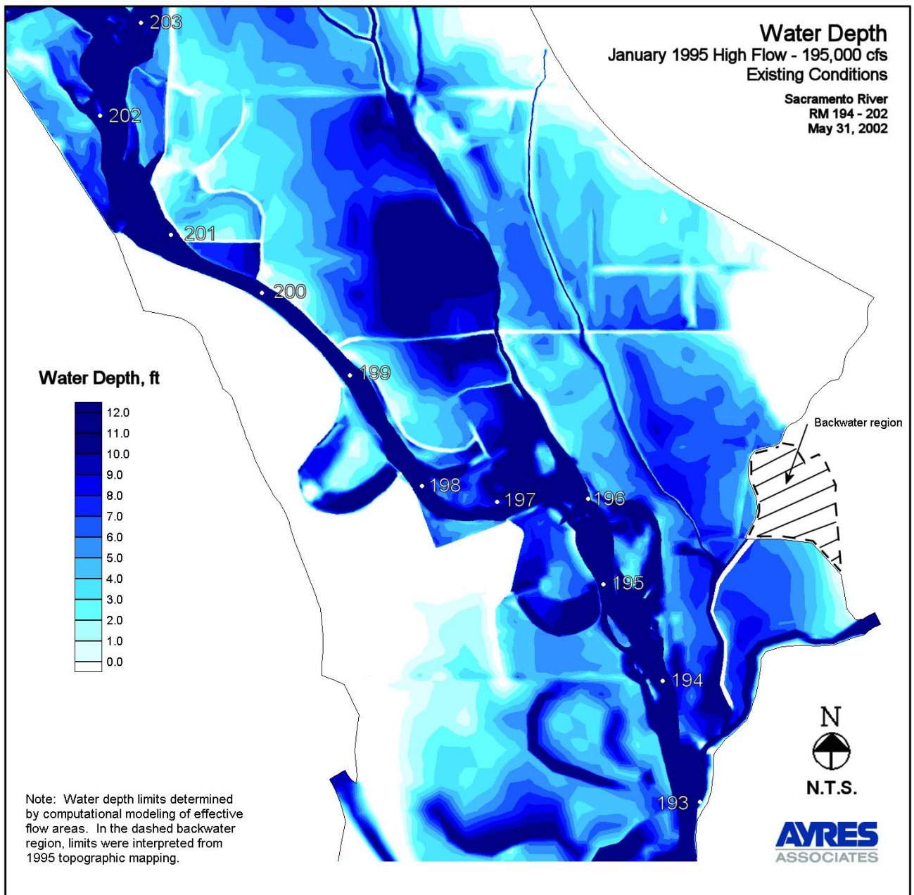
Figure 21. Water Depth - Existing Conditions
