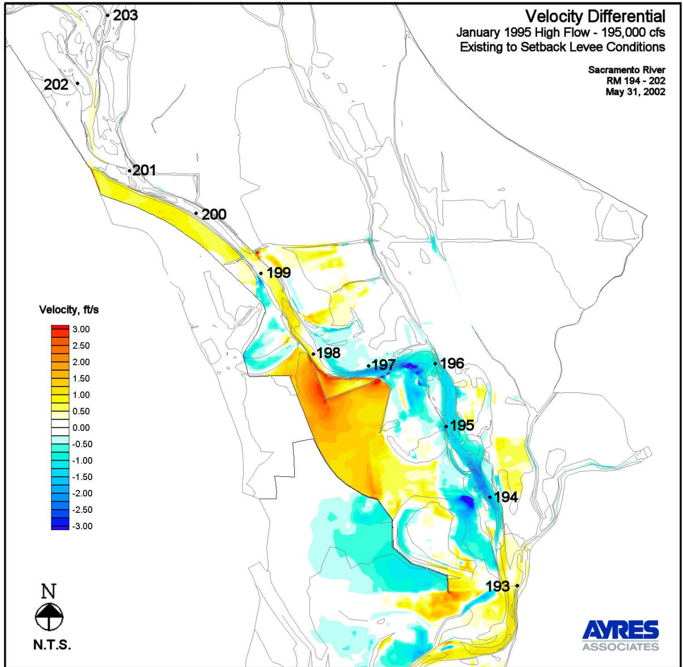
Figure 19. Velocity Diferential - Existing to Setback Levee Conditions
