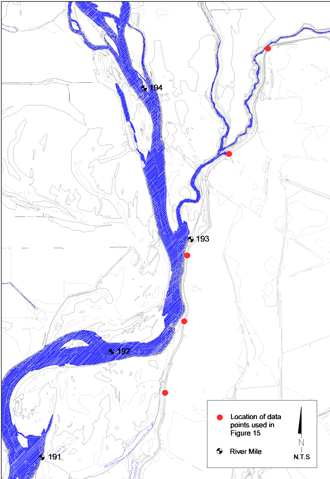
Figure 34. Plan View of East Levee Showing Data Point Locations
