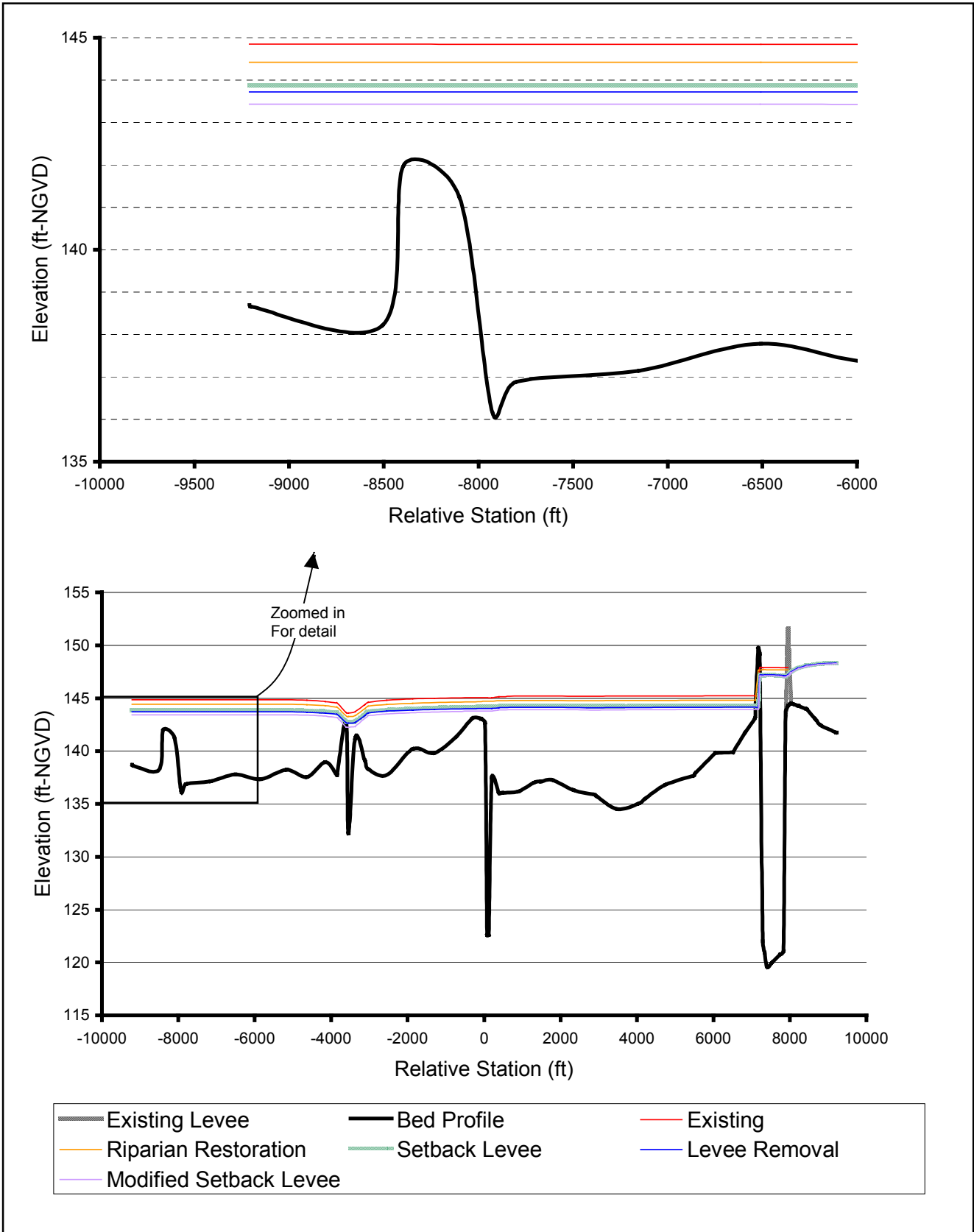
Figure 32. Computed Water Surface Elevations Upstream of Highway 32
