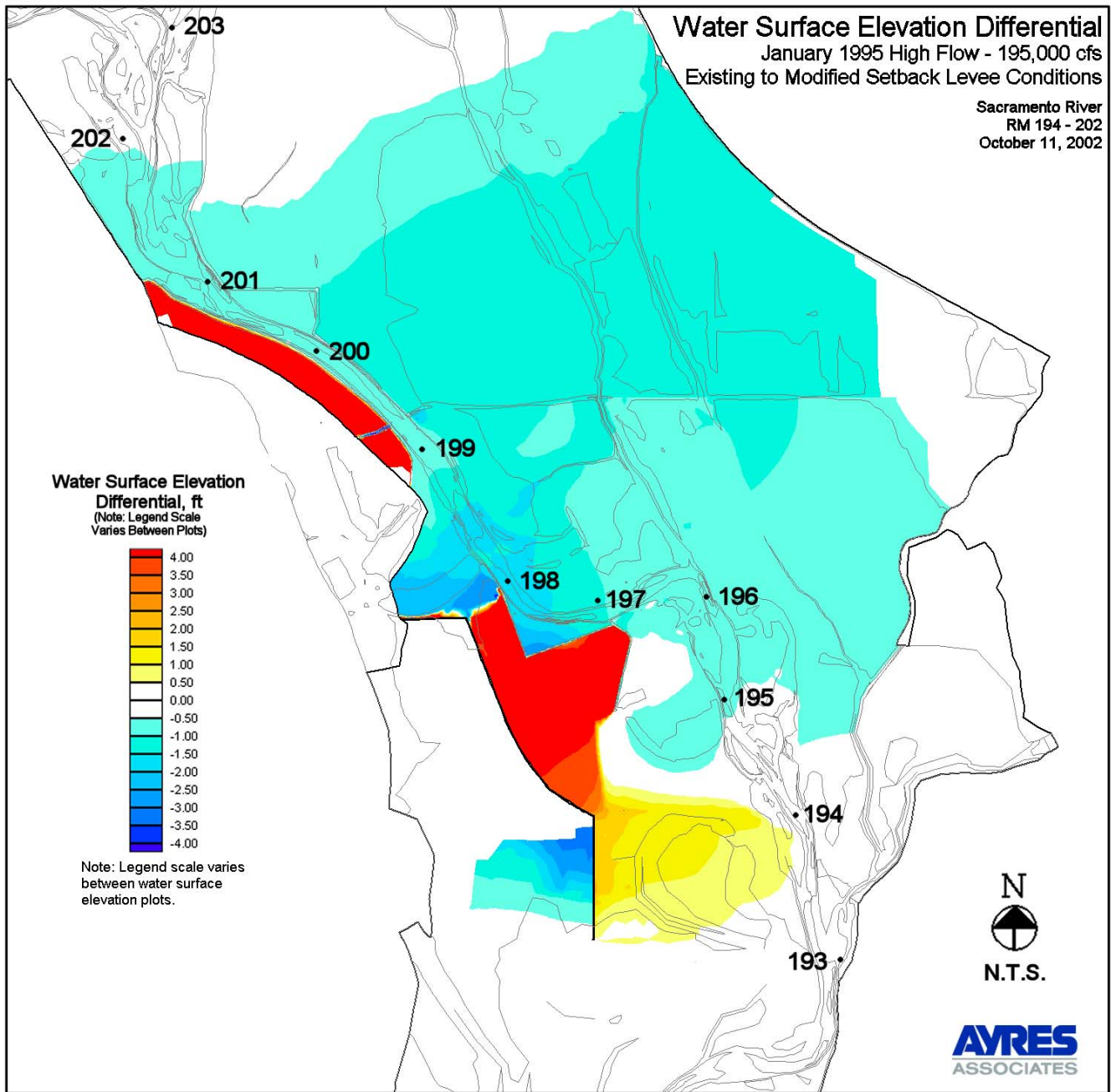
Figure 31. Water Surface Elevation Differential - Existing to Modified Setback Levee Conditions
