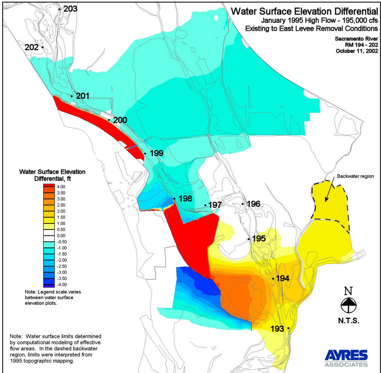
Figure 30. Water Surface Elevation Differential - Existing to East Levee Removal Conditions
