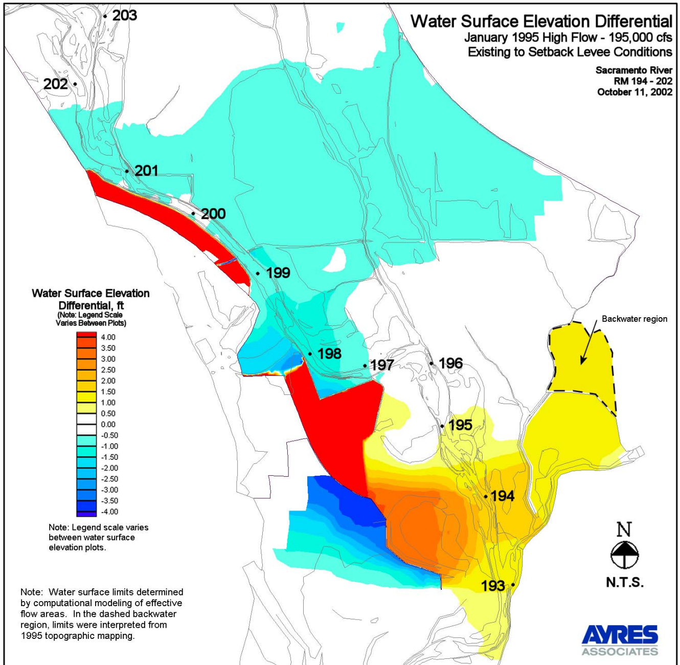
Figure 29. Water Surface Elevation Differential - Existing to Setback Levee Conditions
