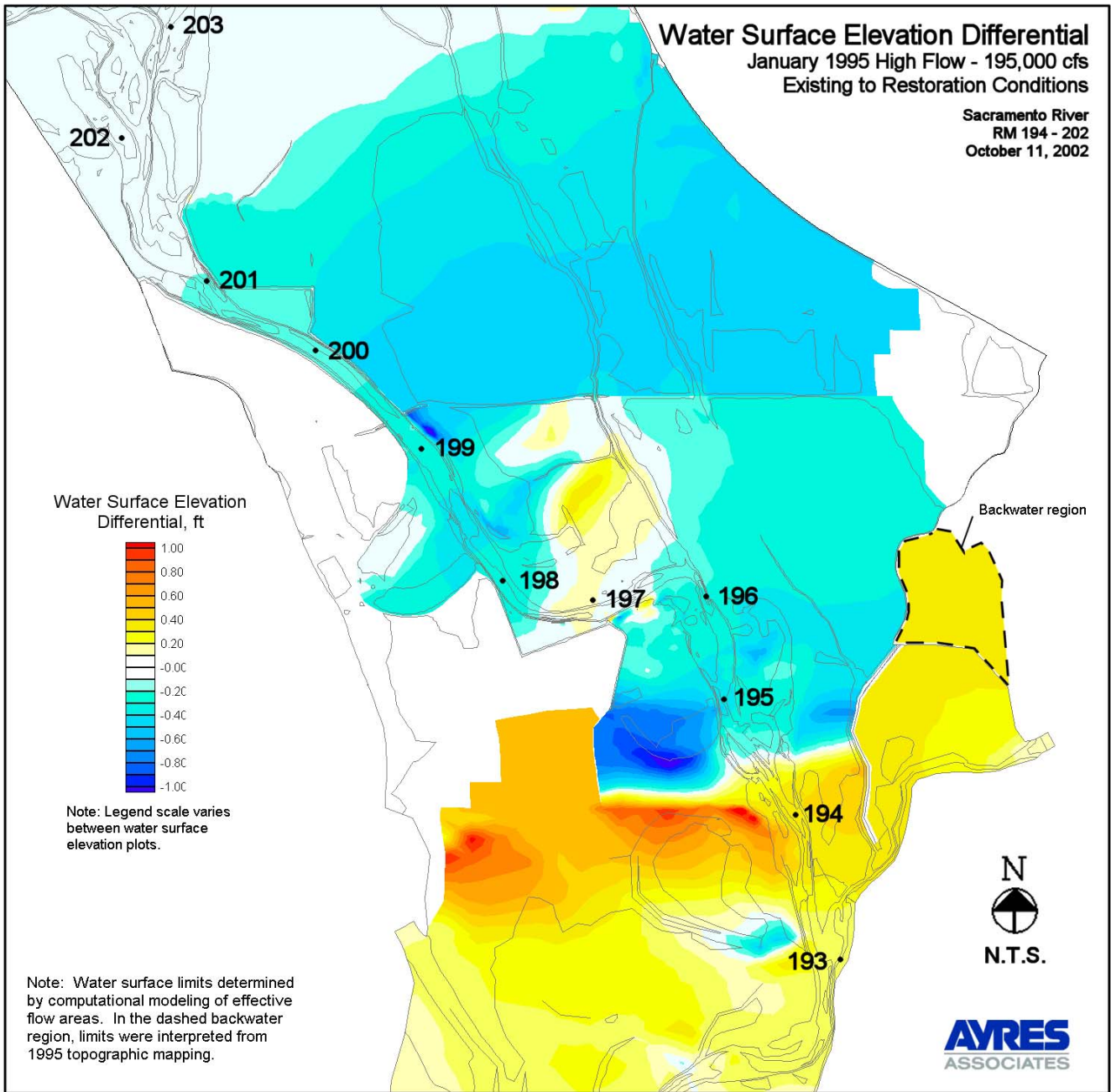
Figure 28. Water Surface Elevation Differential - Existing to Restoration Conditions
