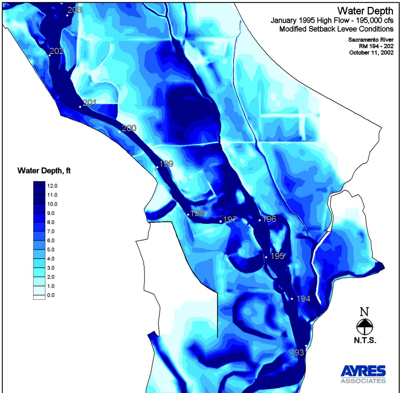
Figure 27. Water Depth - Setback Levee Conditions
