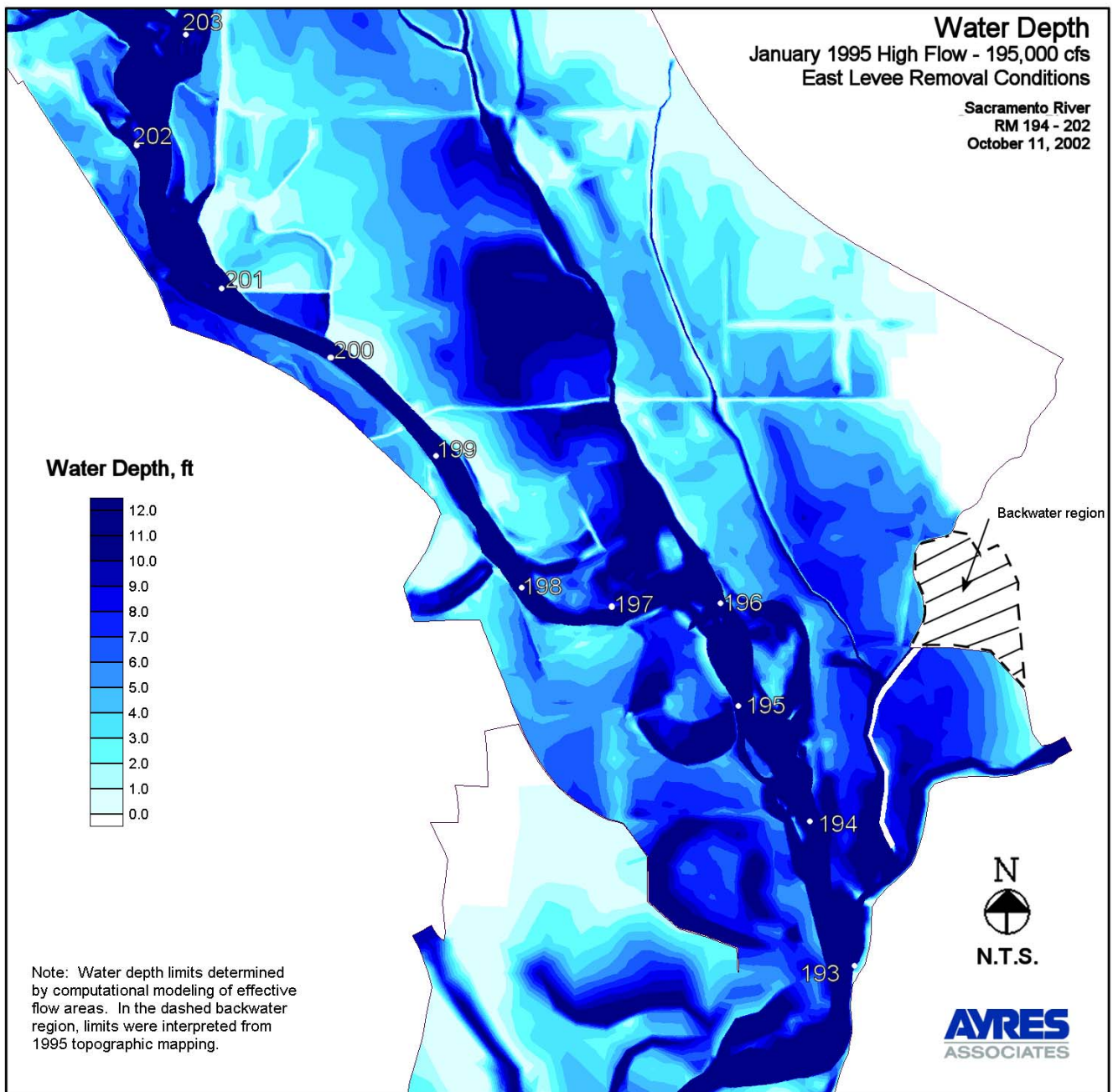
Figure 26. Water Depth - East Levee Removal Conditions
