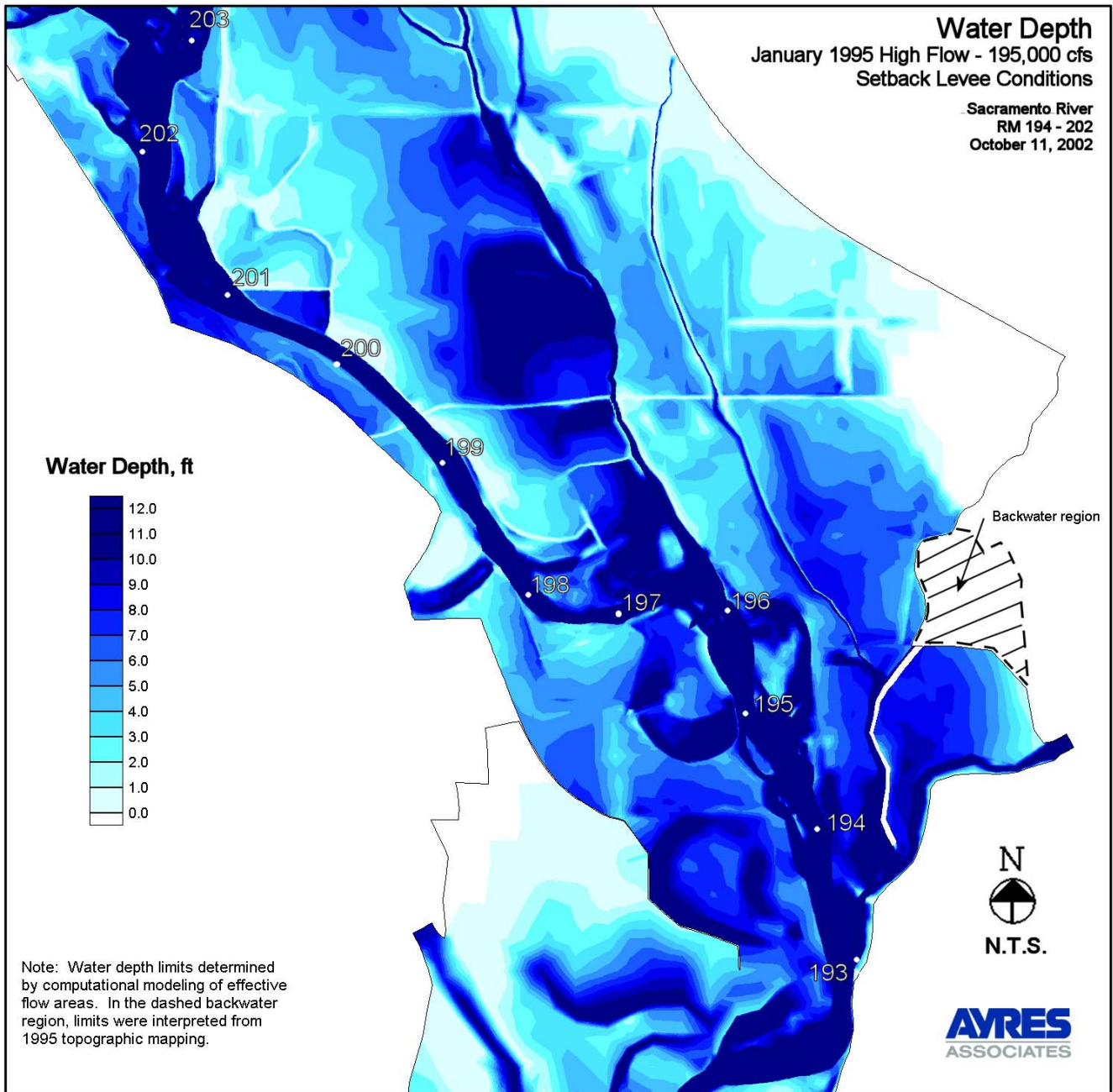
Figure 25. Water Depth - Setback Levee Conditions
