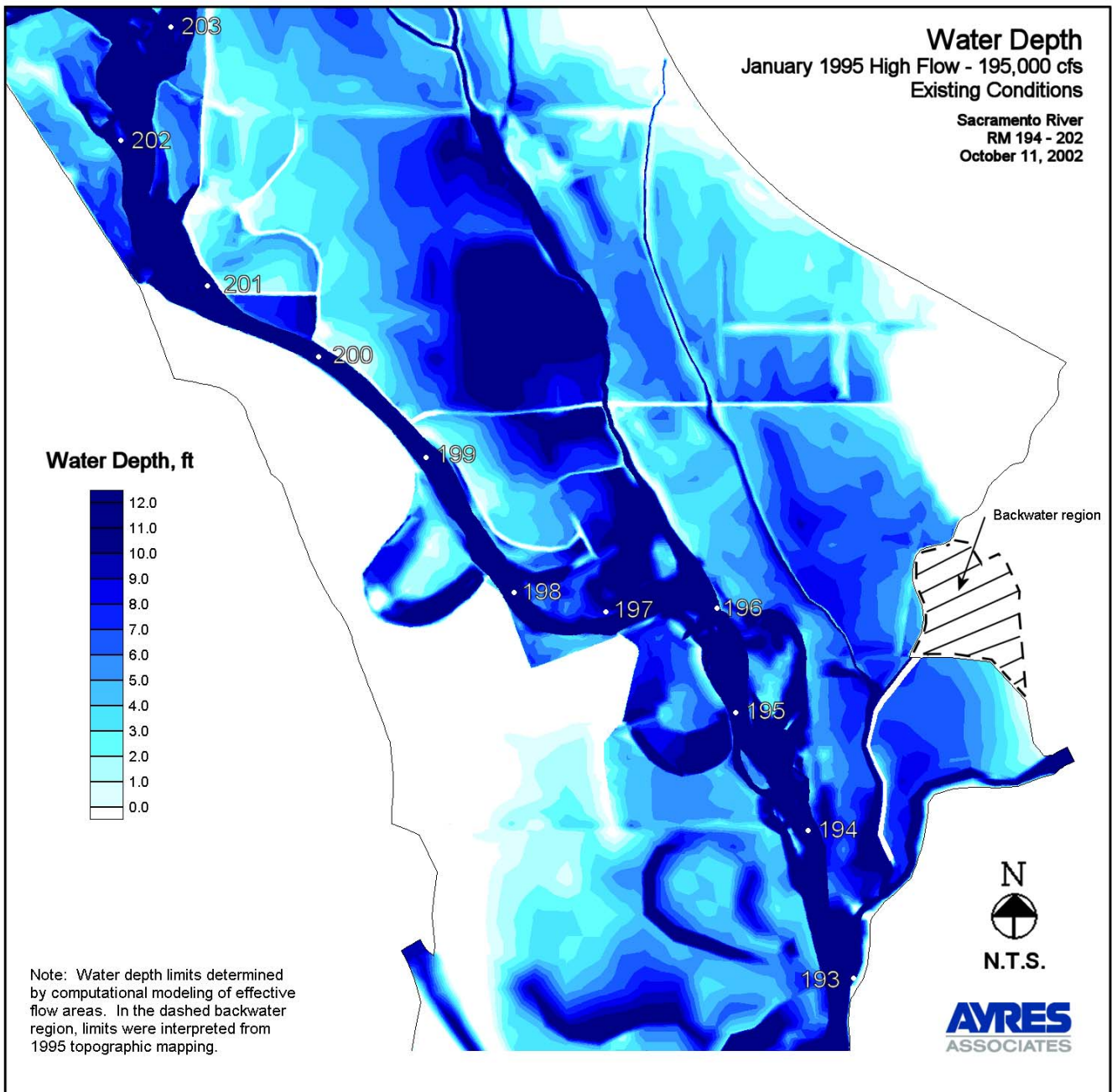
Figure 24. Water Depth - Existing Conditions
