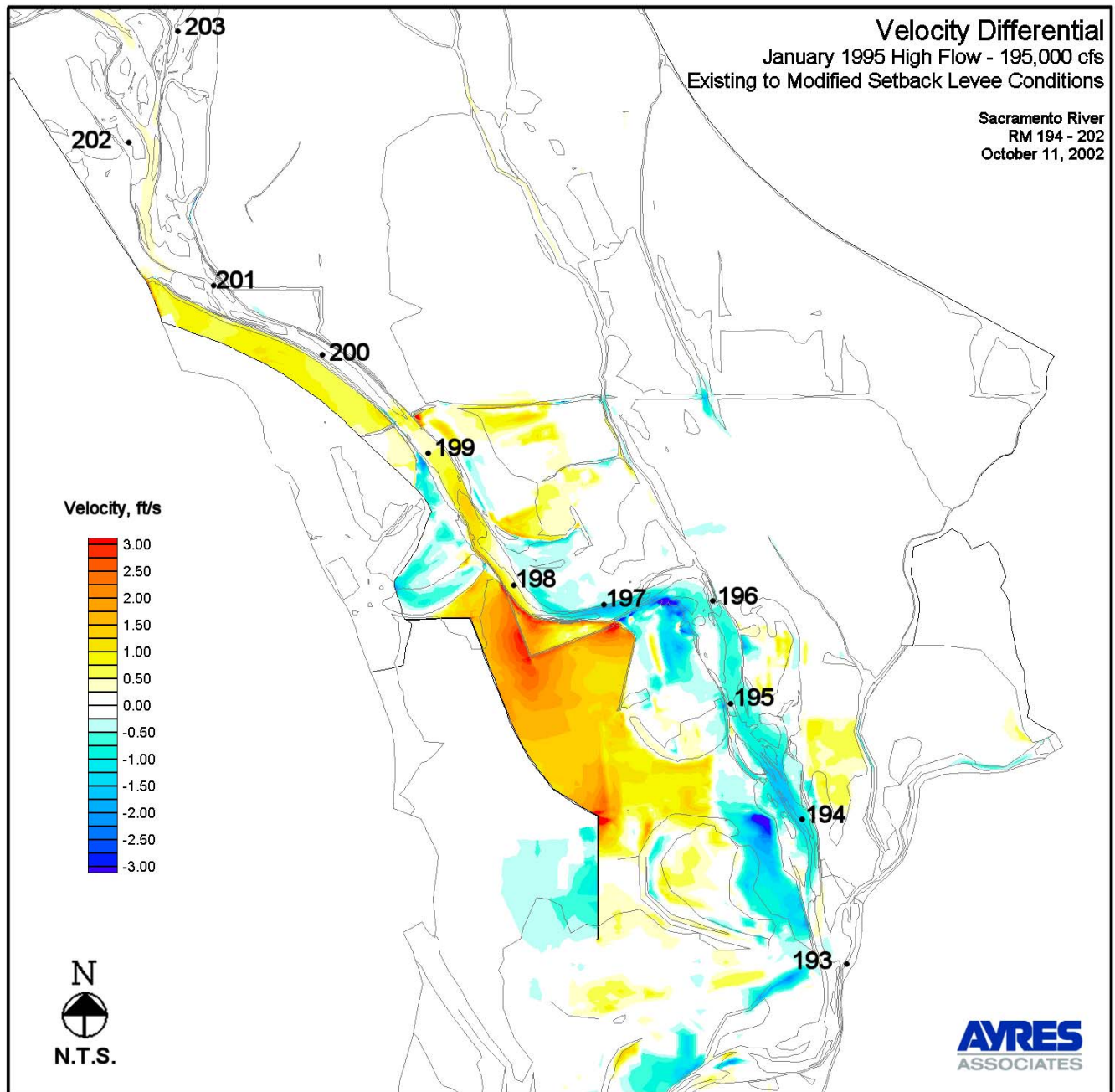
Figure 23. Velocity Diferential - Existing to Modified Setback Levee Conditions
