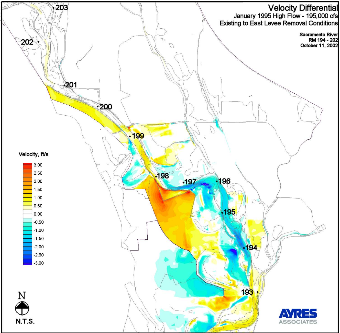
Figure 22. Velocity Diferential - Existing to East Levee Removal Conditions
