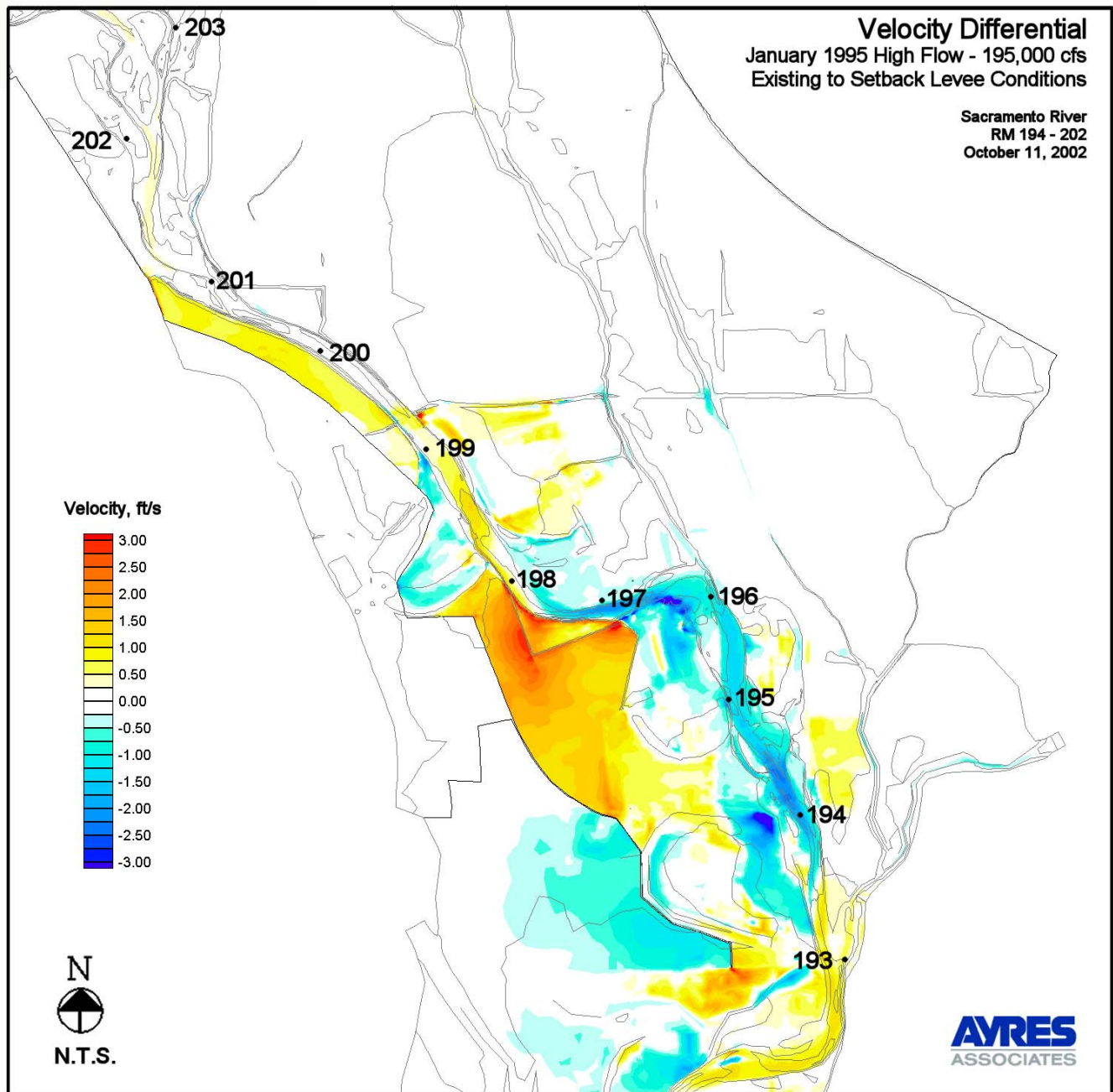
Figure 21. Velocity Diferential - Existing to Setback Levee Conditions
