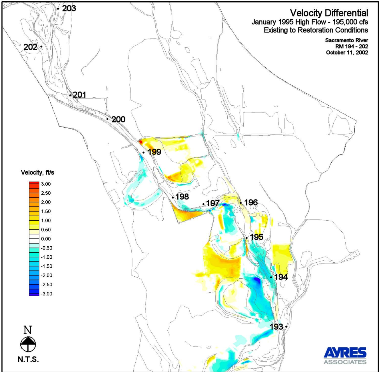
Figure 20. Velocity Differential - Existing to Restoration Conditions
