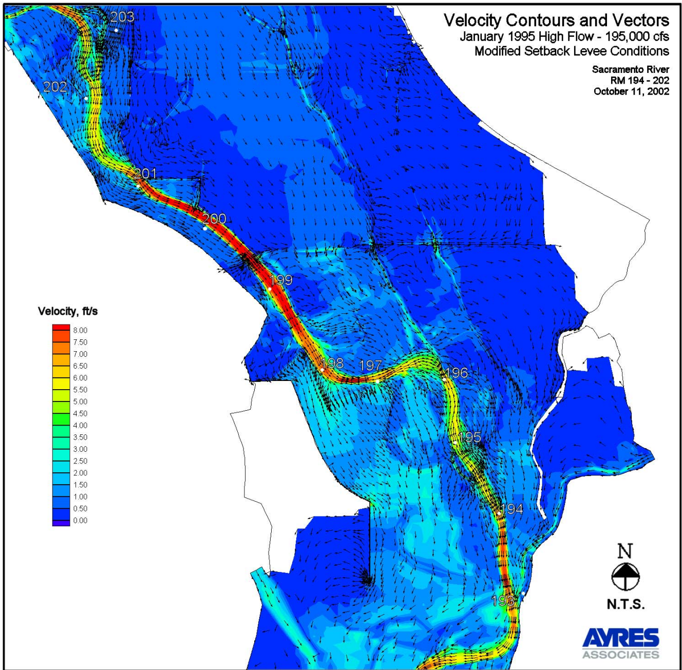
Figure 19. Velocity Contours and Vectors - Modified Setback Levee Conditions
