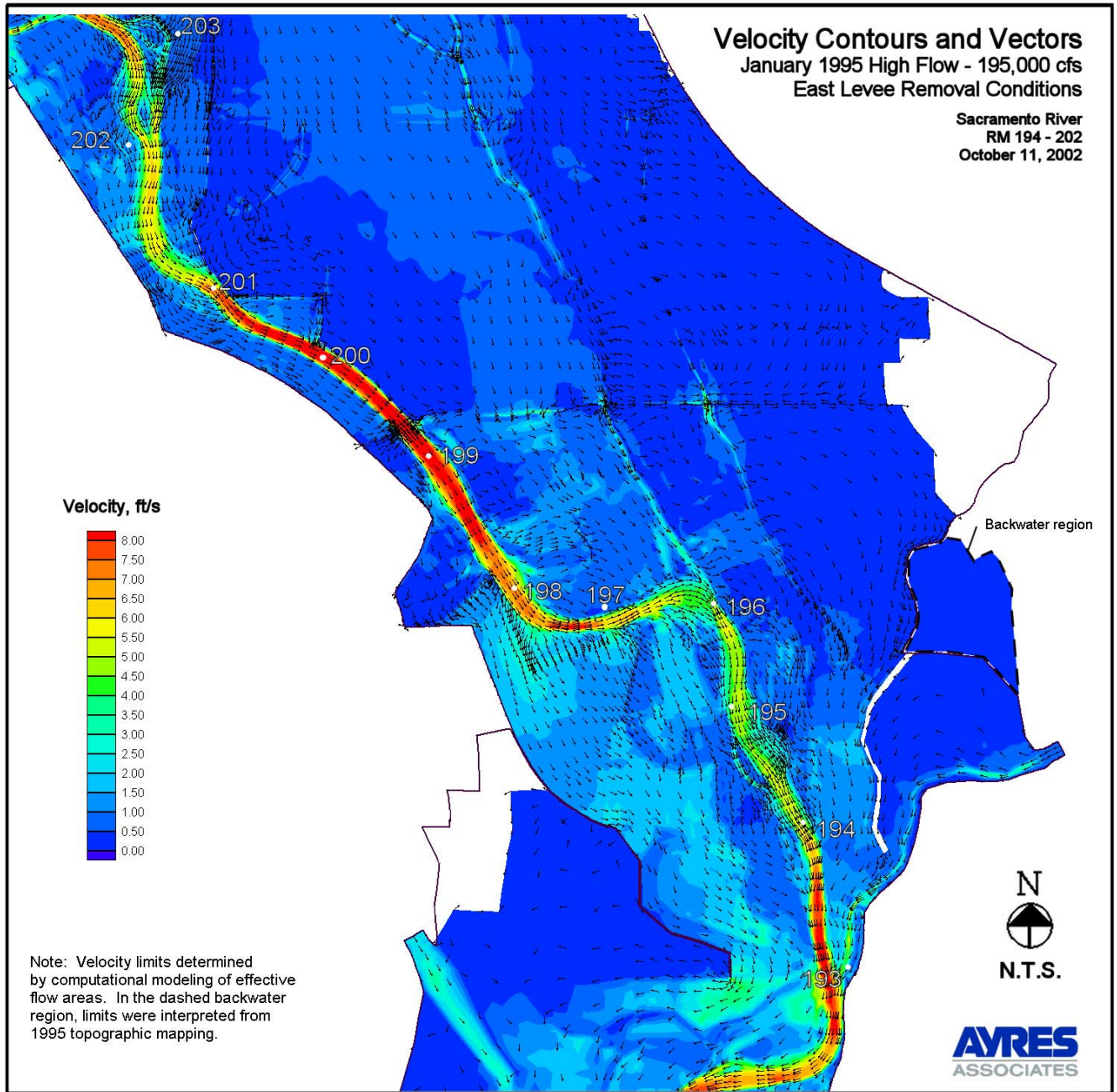
Figure 18. Velocity Contours and Vectors - East Levee Removal Conditions
