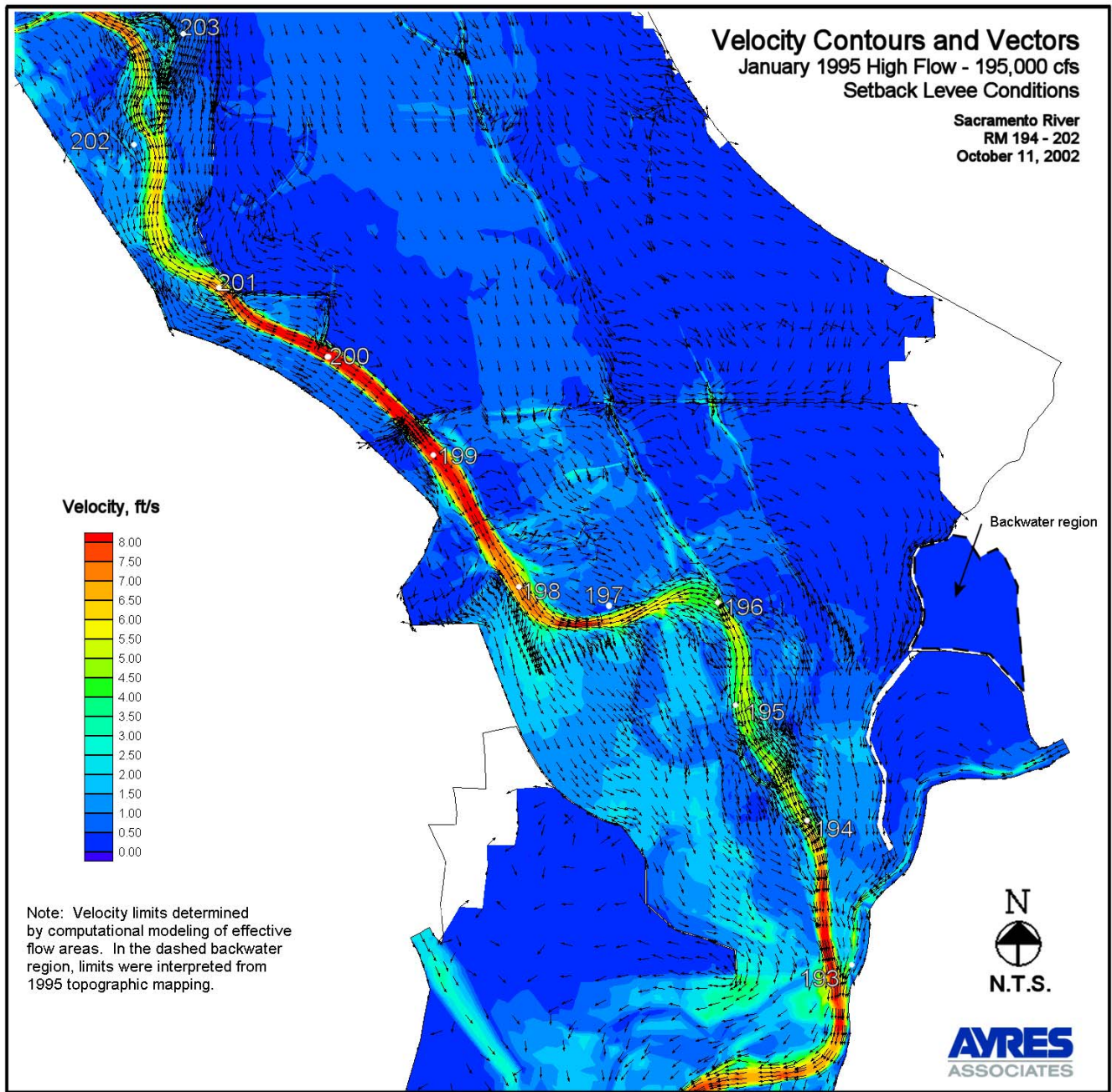
Figure 17. Velocity Contours and Vectors - Setback Levee Conditions
