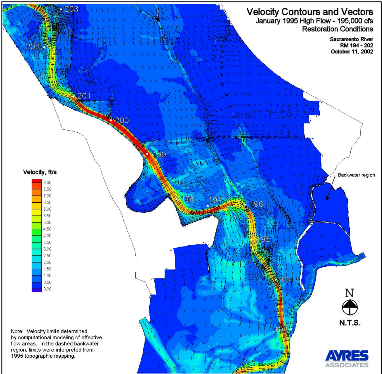
Figure 16. Velocity Contours and Vectors - Restoration Conditions
