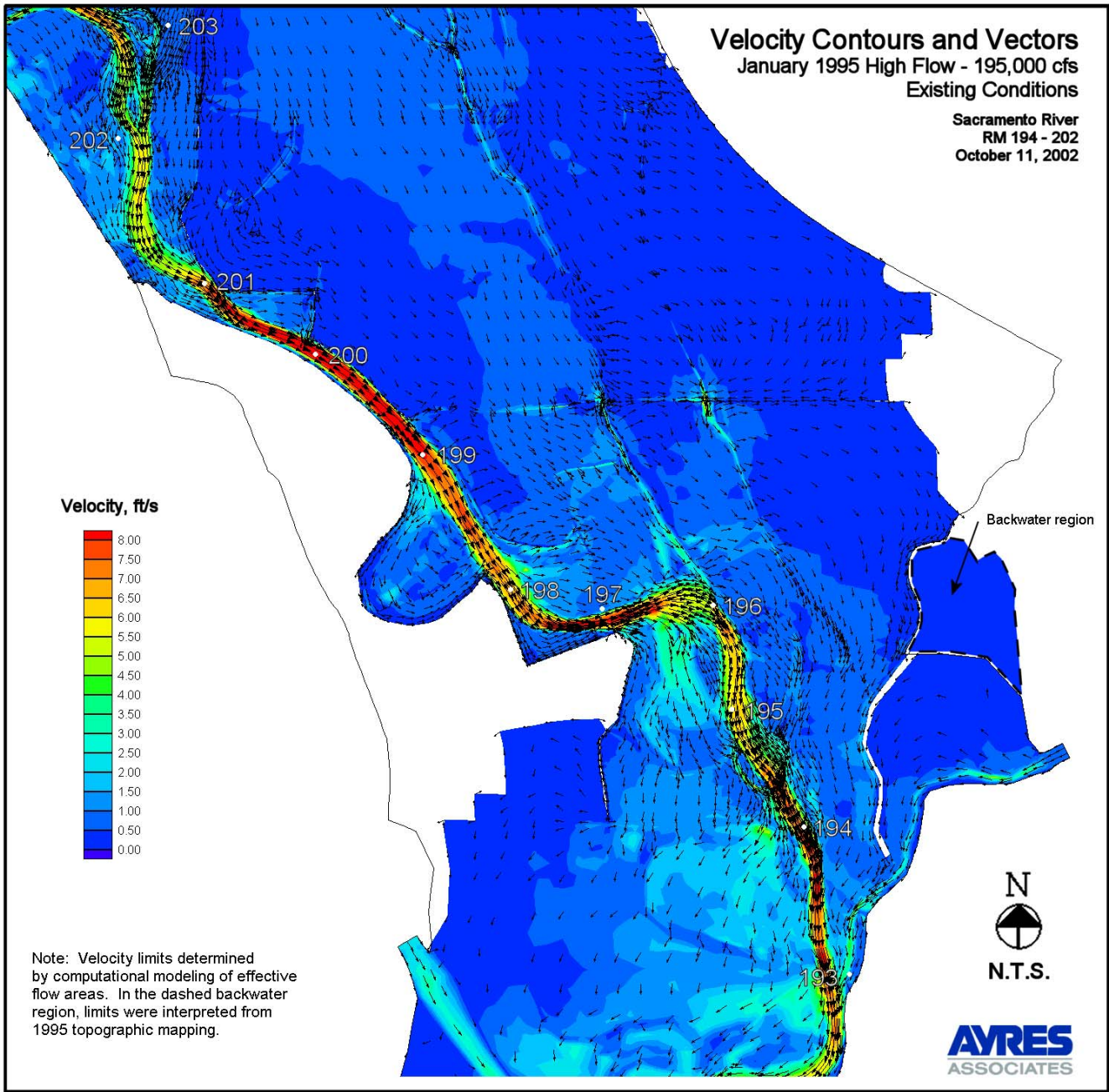
Figure 15. Velocity Contours and Vectors - Existing Conditions
