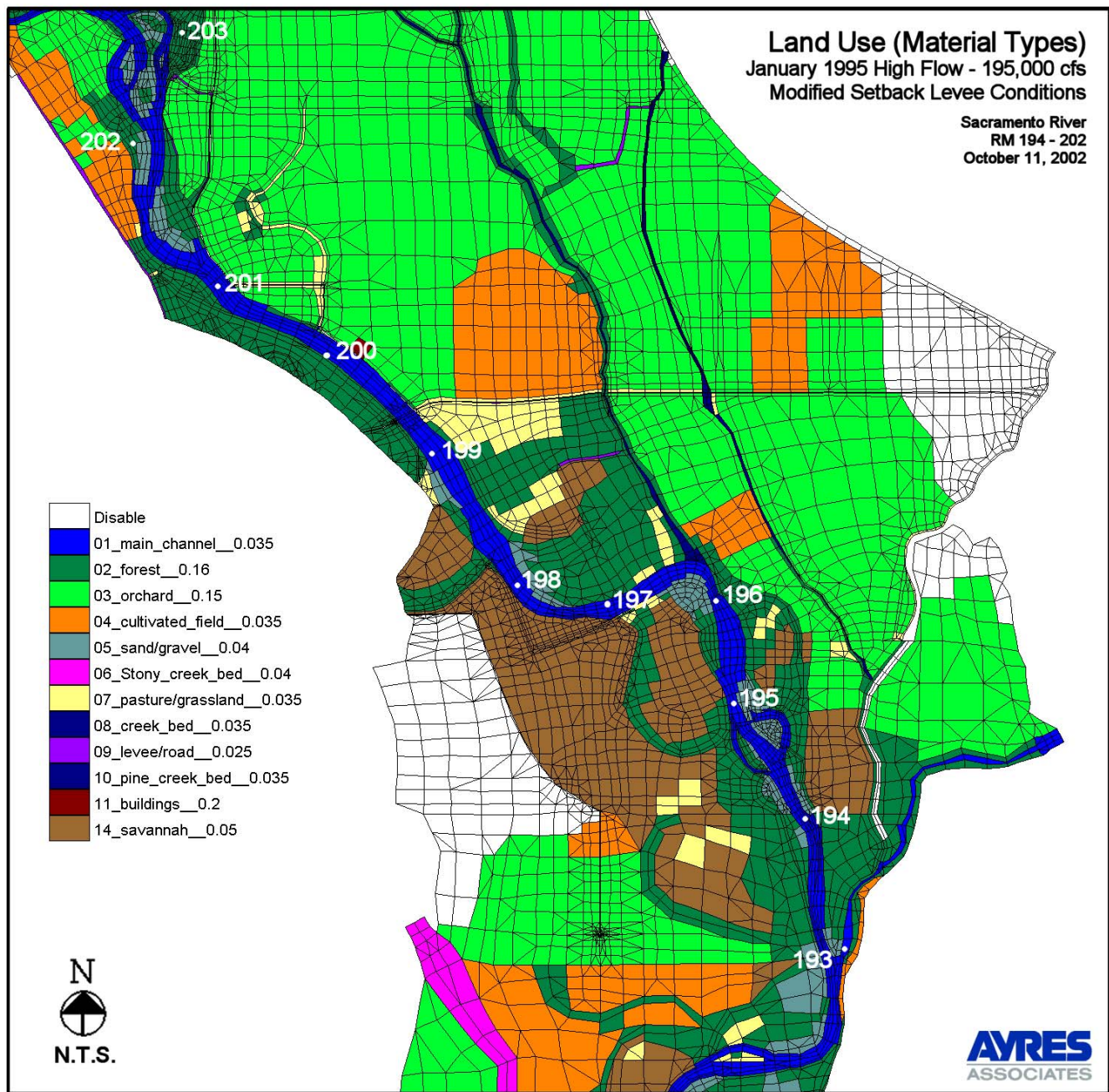
Figure 14. Land Use/Material Types - Modified Setback Levee Conditions
