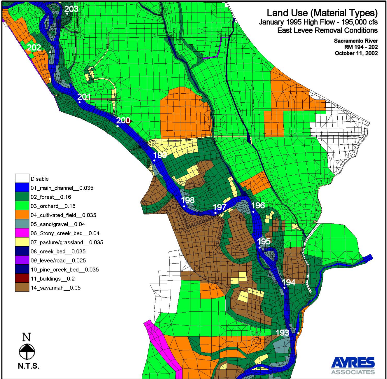
Figure 13. Land Use/Material Types - East Levee Removal Conditions
