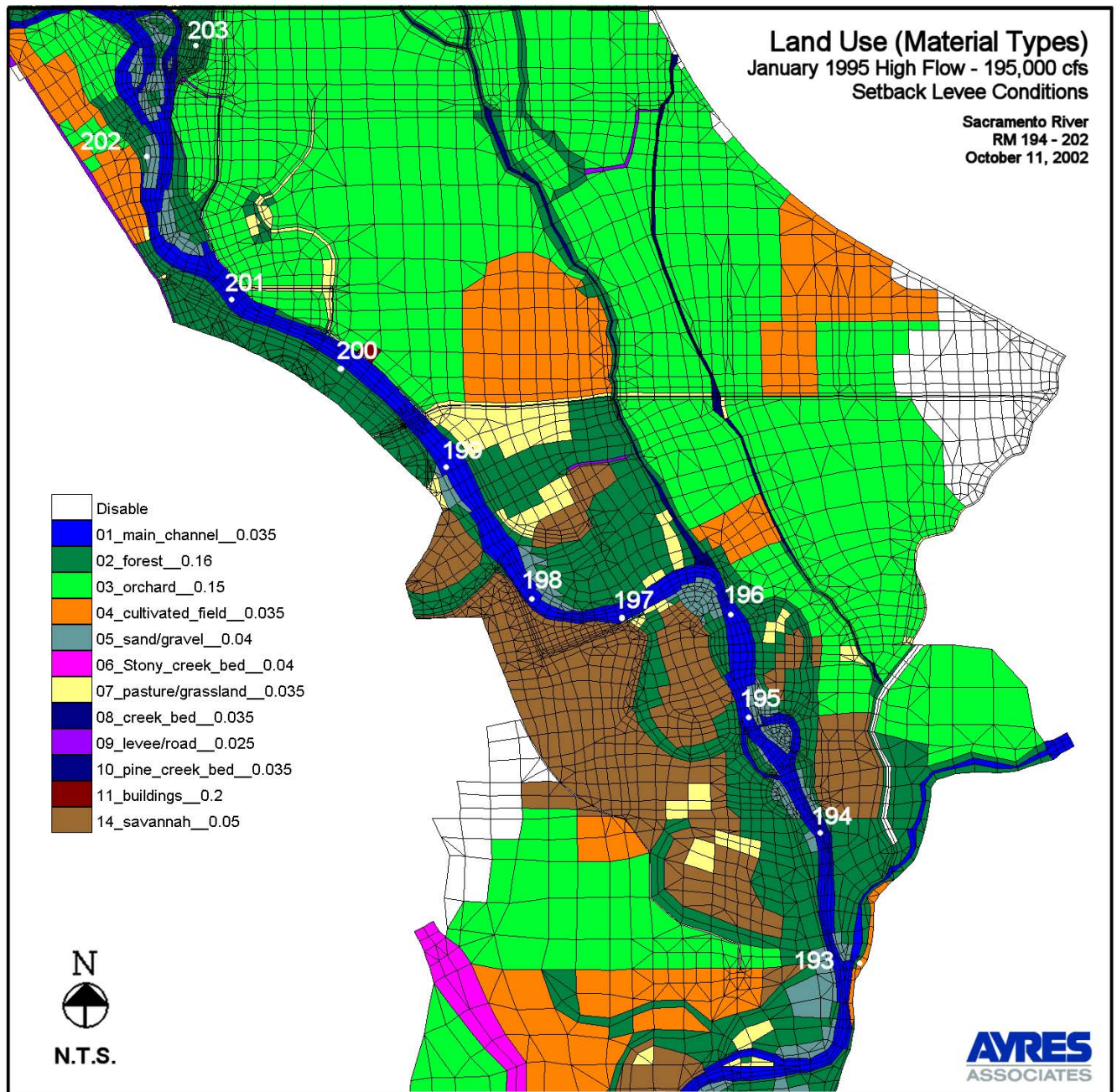
Figure 12. Land Use/Material Types - Setback Levee Conditions
