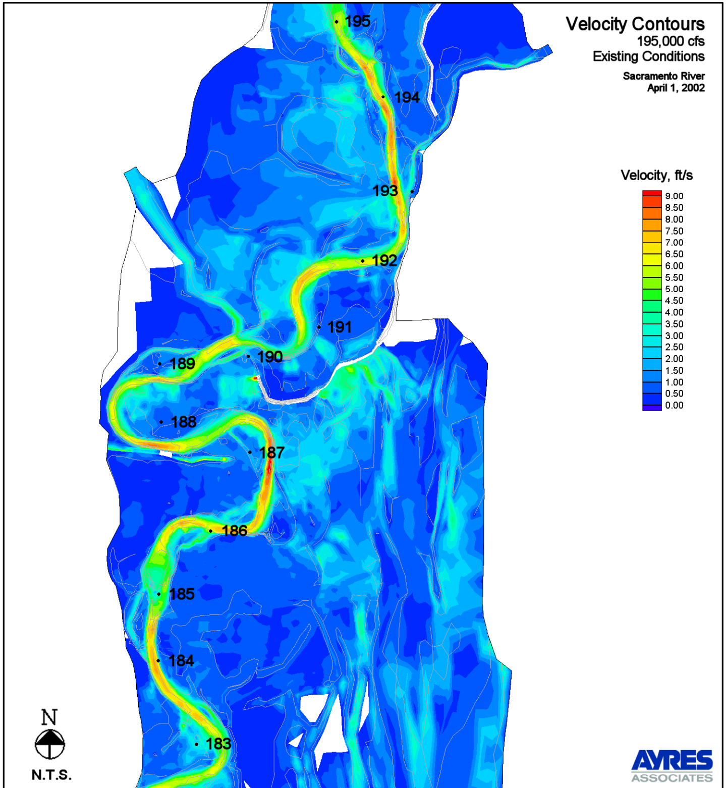
Figure 9. Velocity Contours - Existing Conditions - 195,000 cfs
