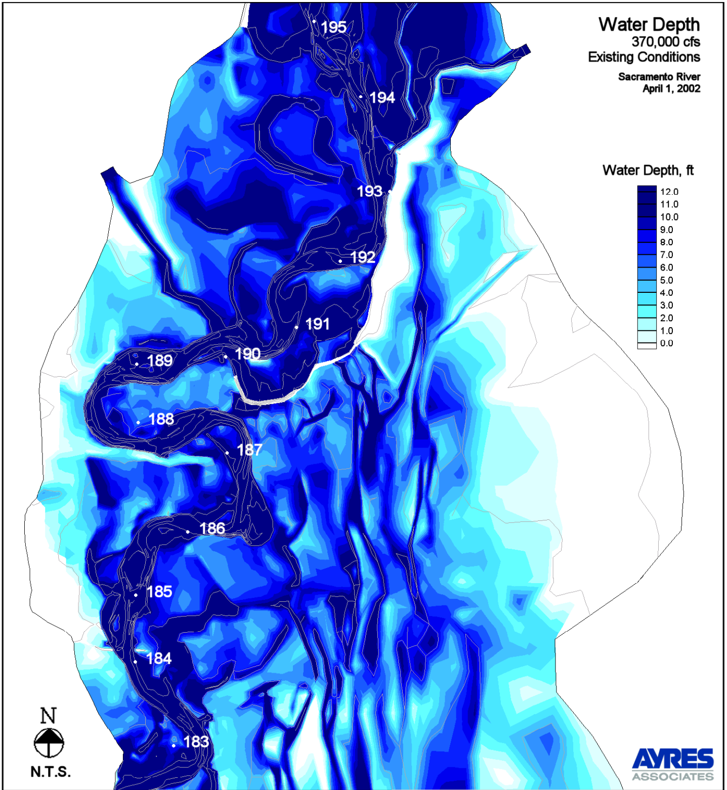
Figure 8. Water Depth - Existing Conditions - 370,000 cfs
