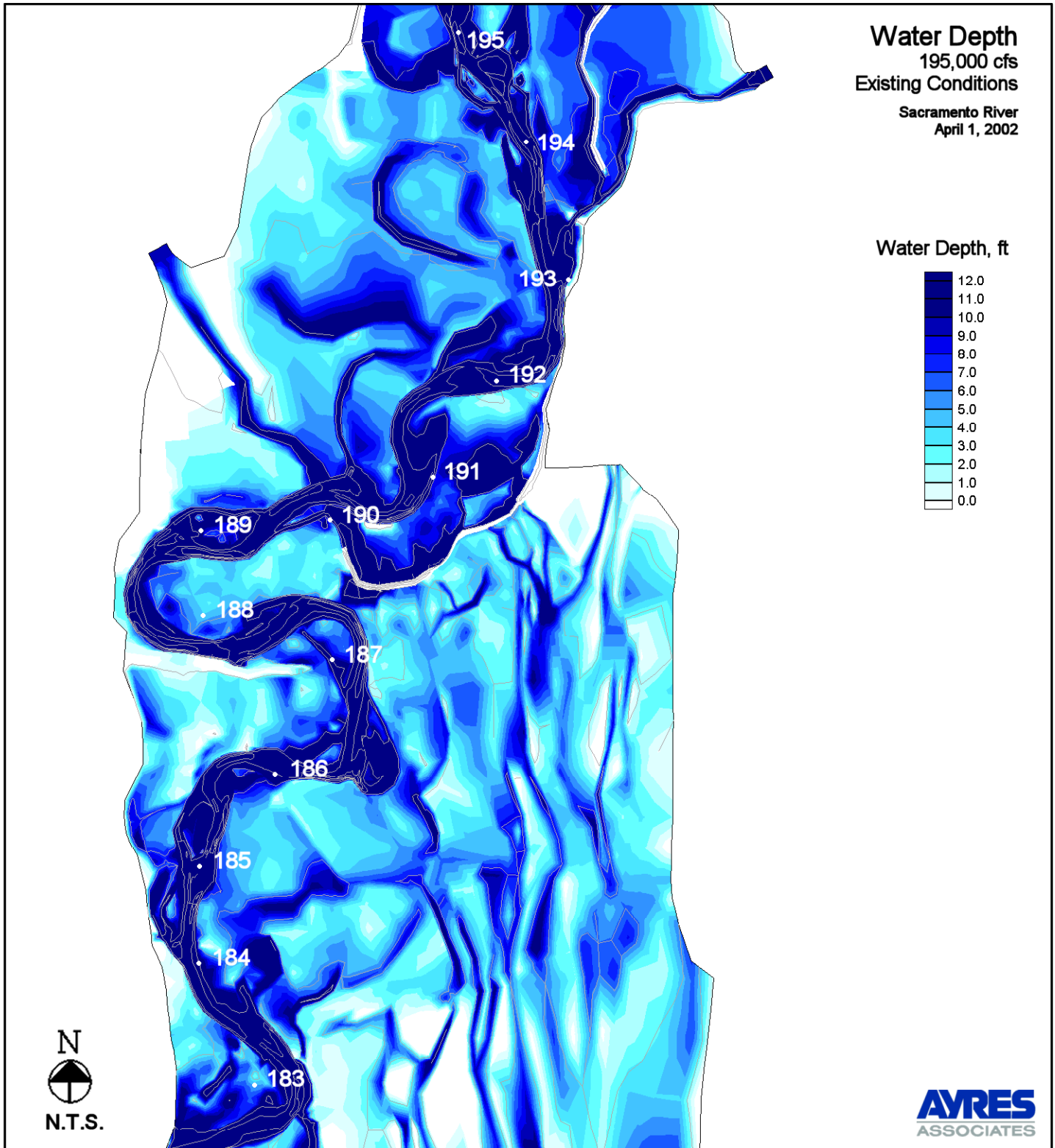
Figure 7. Water Depth - Existing Conditions - 195,000 cfs
